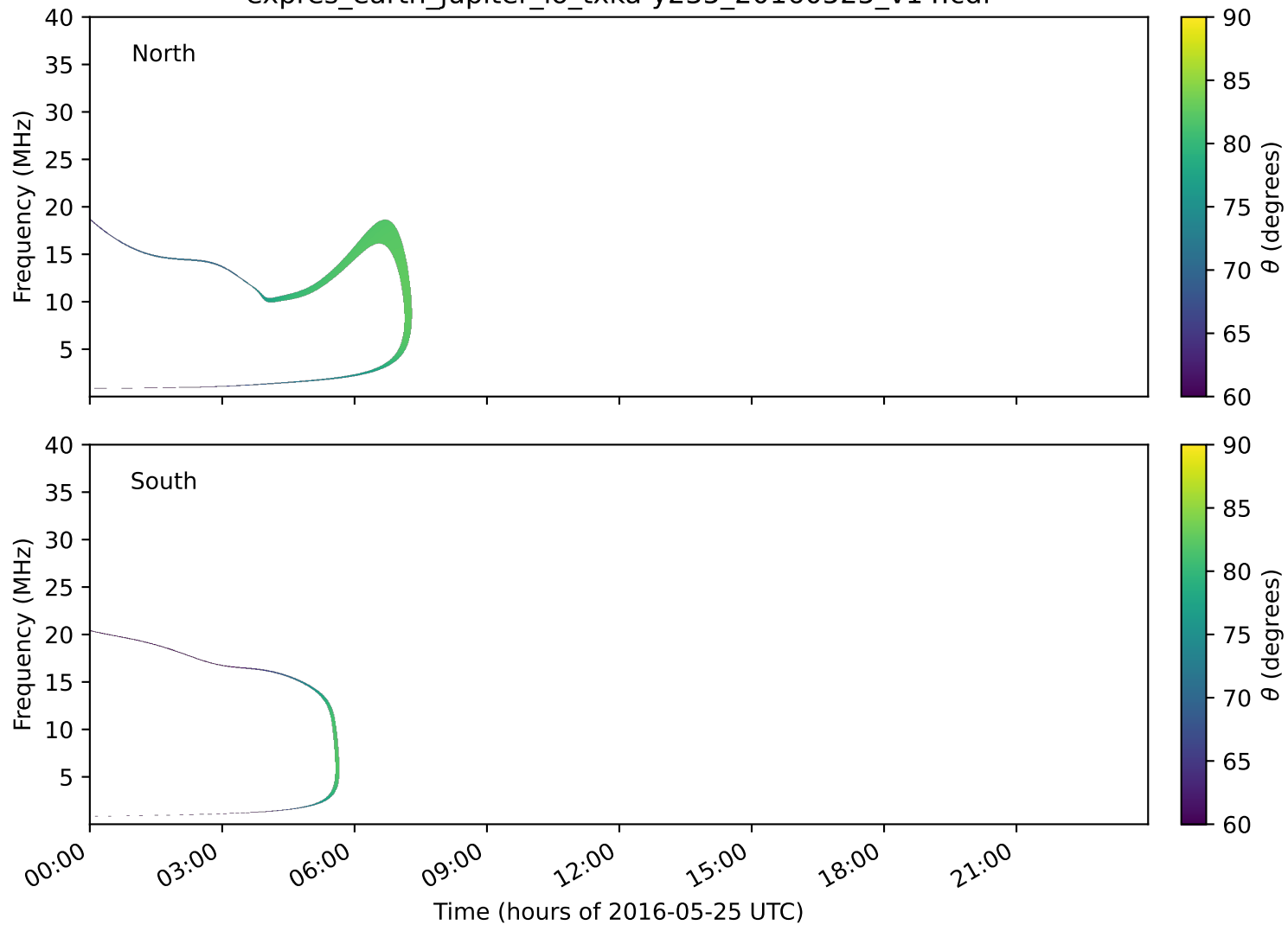
expres_earth_jupiter_io_txka-y235_20160525_v14.cdf
