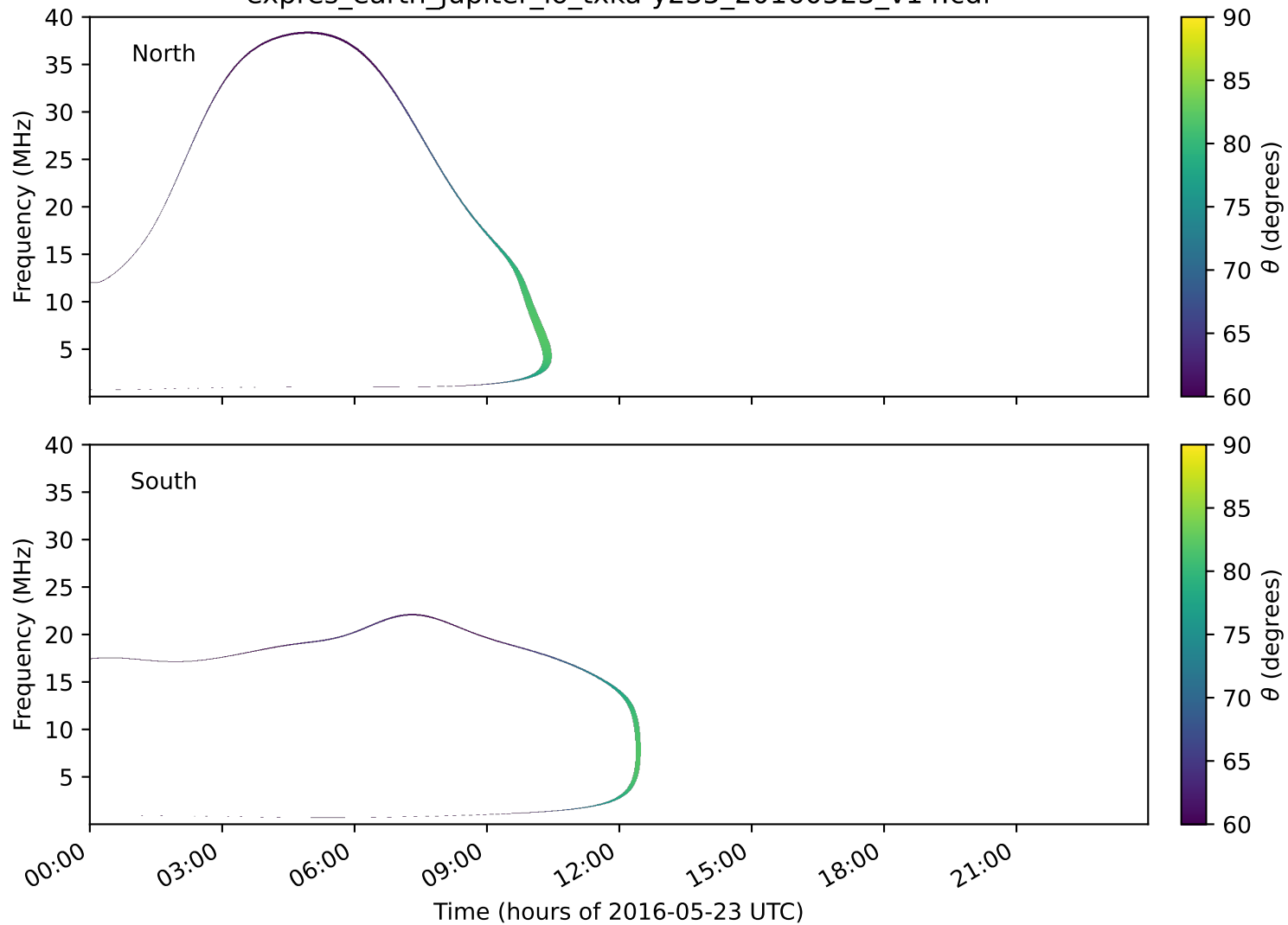
expres_earth_jupiter_io_txka-y235_20160523_v14.cdf
