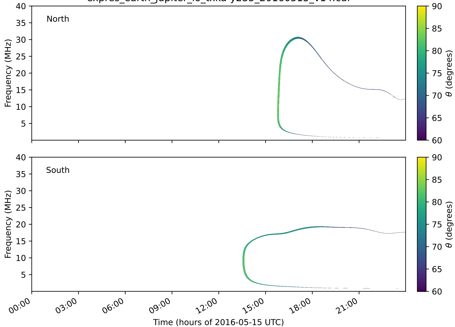
expres_earth_jupiter_io_txka-y235_20160515_v14.cdf
