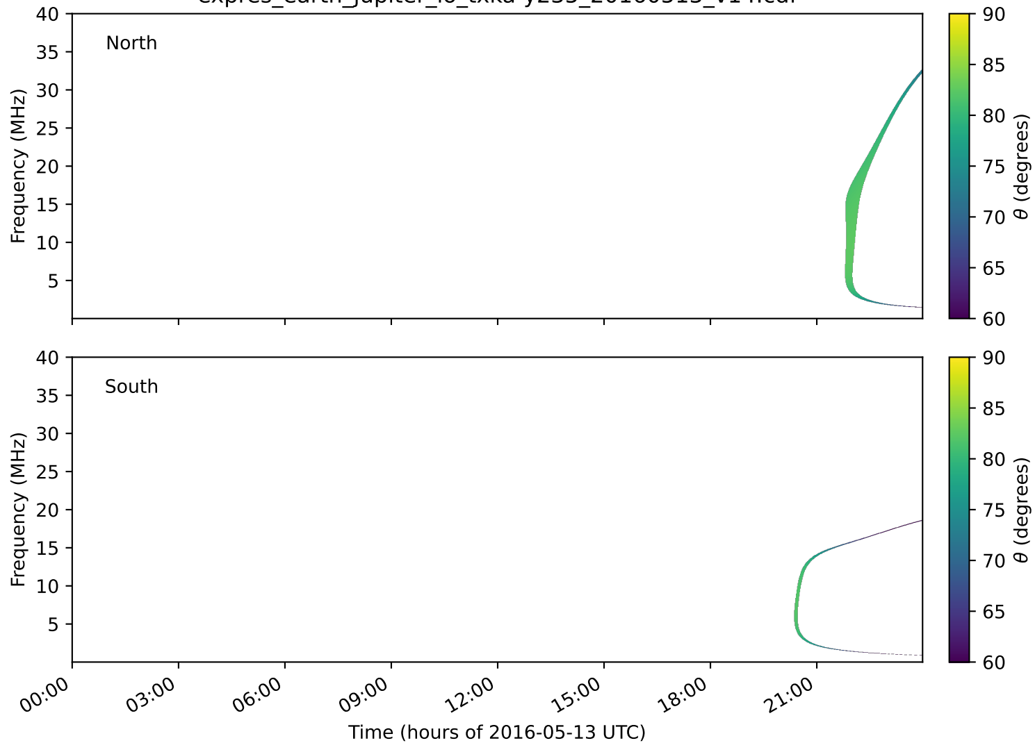
expres_earth_jupiter_io_txka-y235_20160513_v14.cdf
