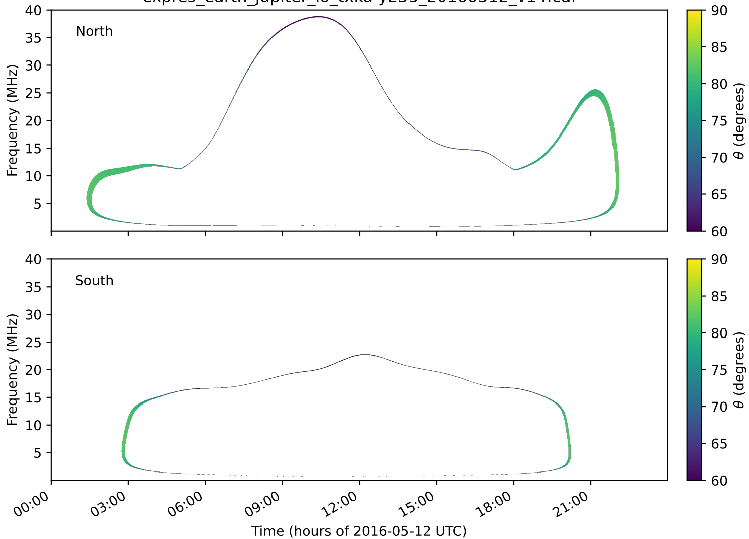
expres_earth_jupiter_io_txka-y235_20160512_v14.cdf
