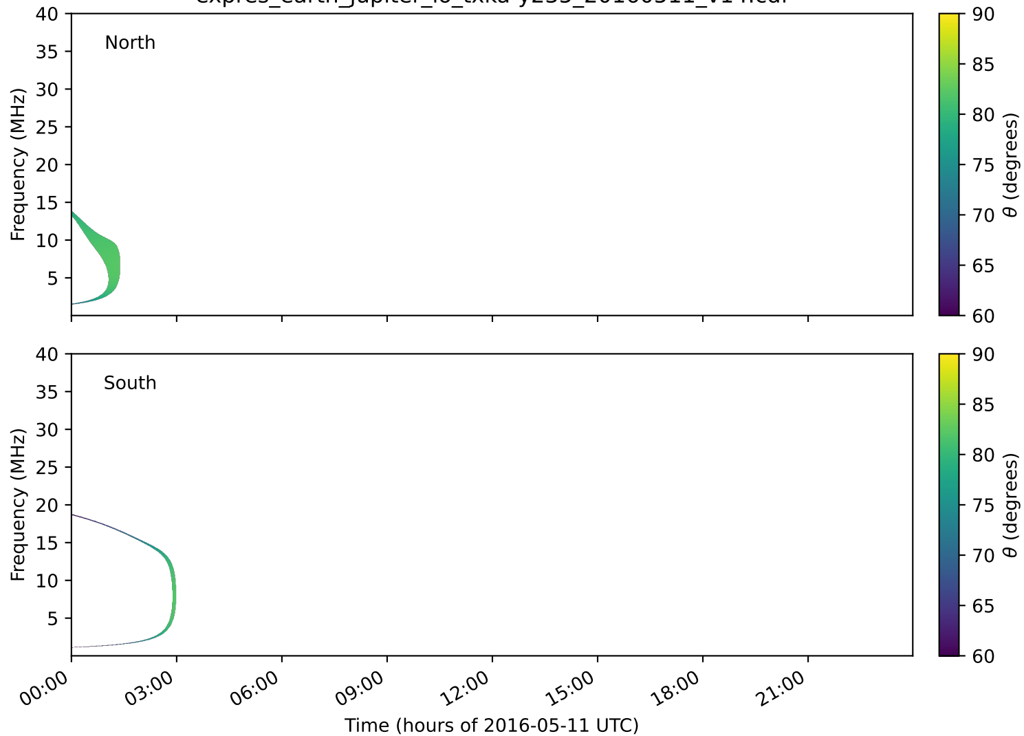
expres_earth_jupiter_io_txka-y235_20160511_v14.cdf
