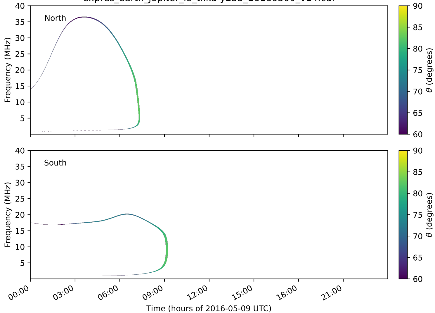
expres_earth_jupiter_io_txka-y235_20160509_v14.cdf
