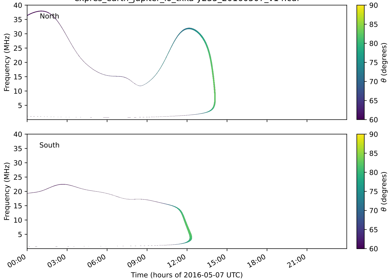
expres_earth_jupiter_io_txka-y235_20160507_v14.cdf
