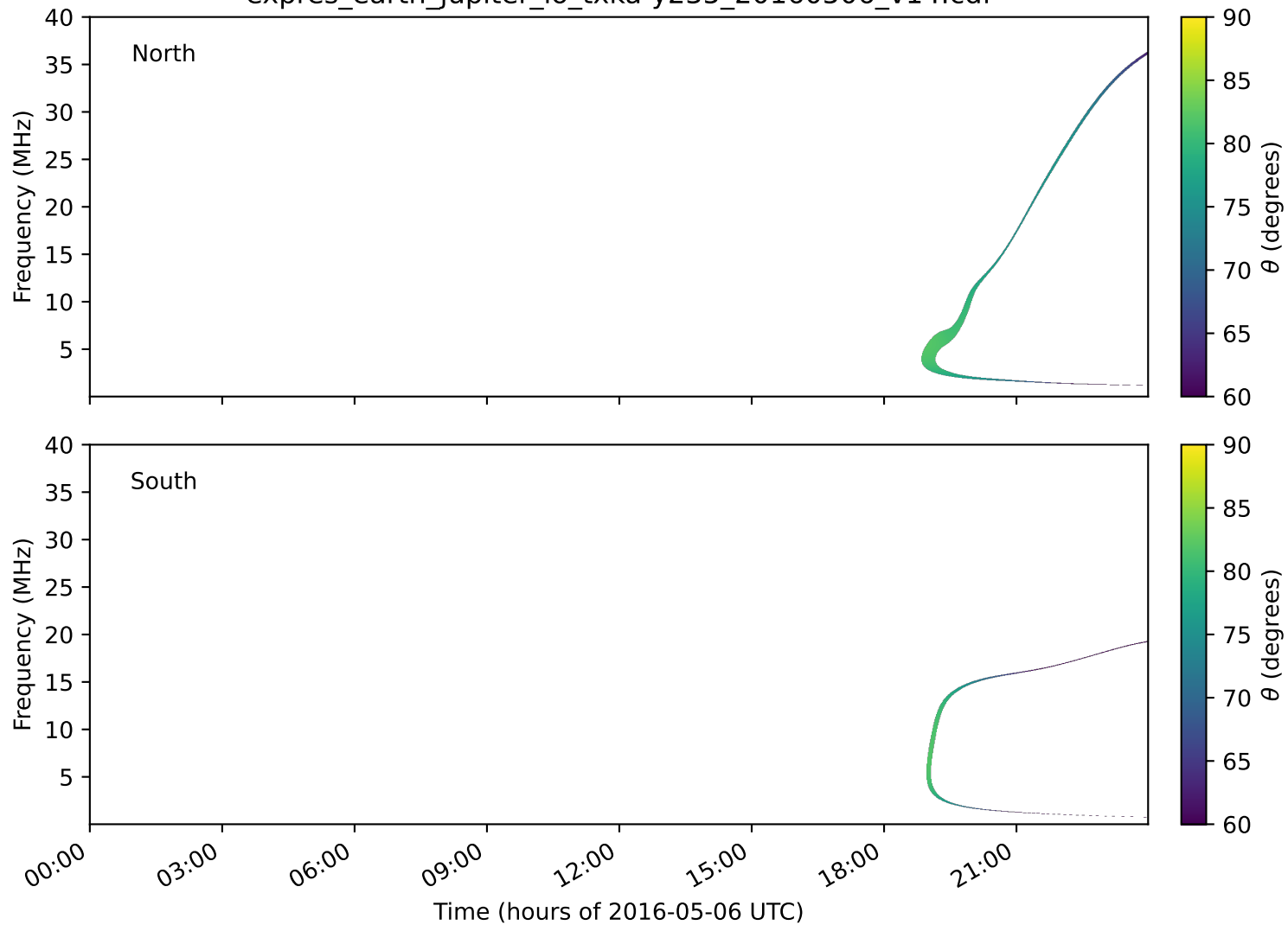
expres_earth_jupiter_io_txka-y235_20160506_v14.cdf
