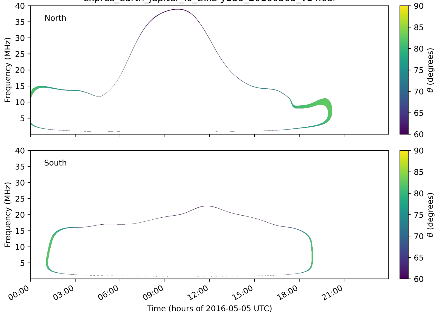
expres_earth_jupiter_io_txka-y235_20160505_v14.cdf
