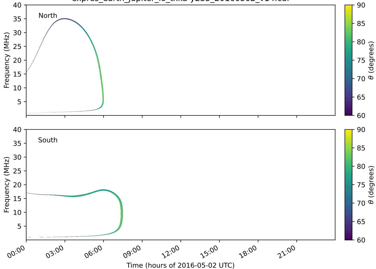
expres_earth_jupiter_io_txka-y235_20160502_v14.cdf
