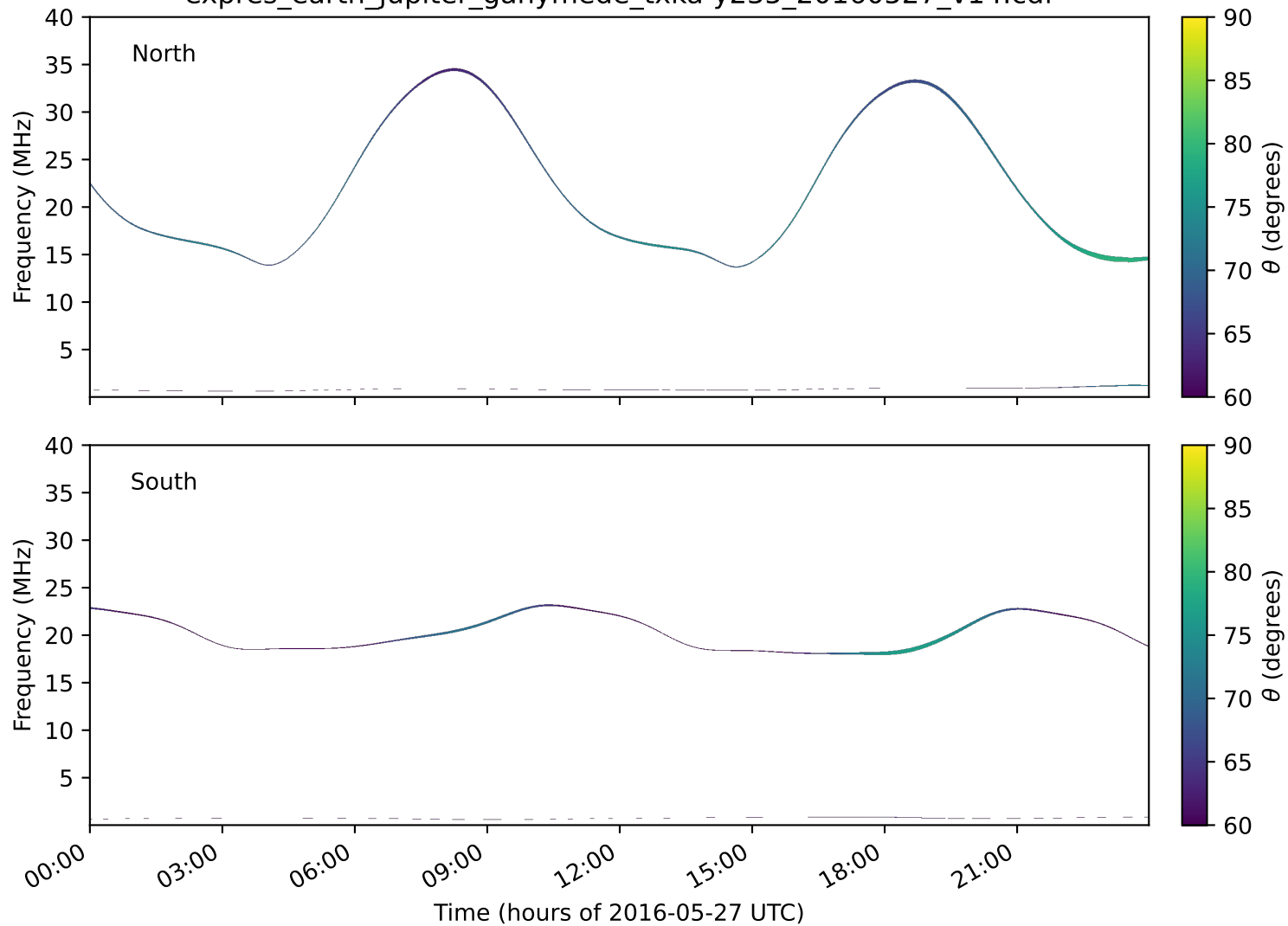
expres_earth_jupiter_ganymede_txka-y235_20160527_v14.cdf
