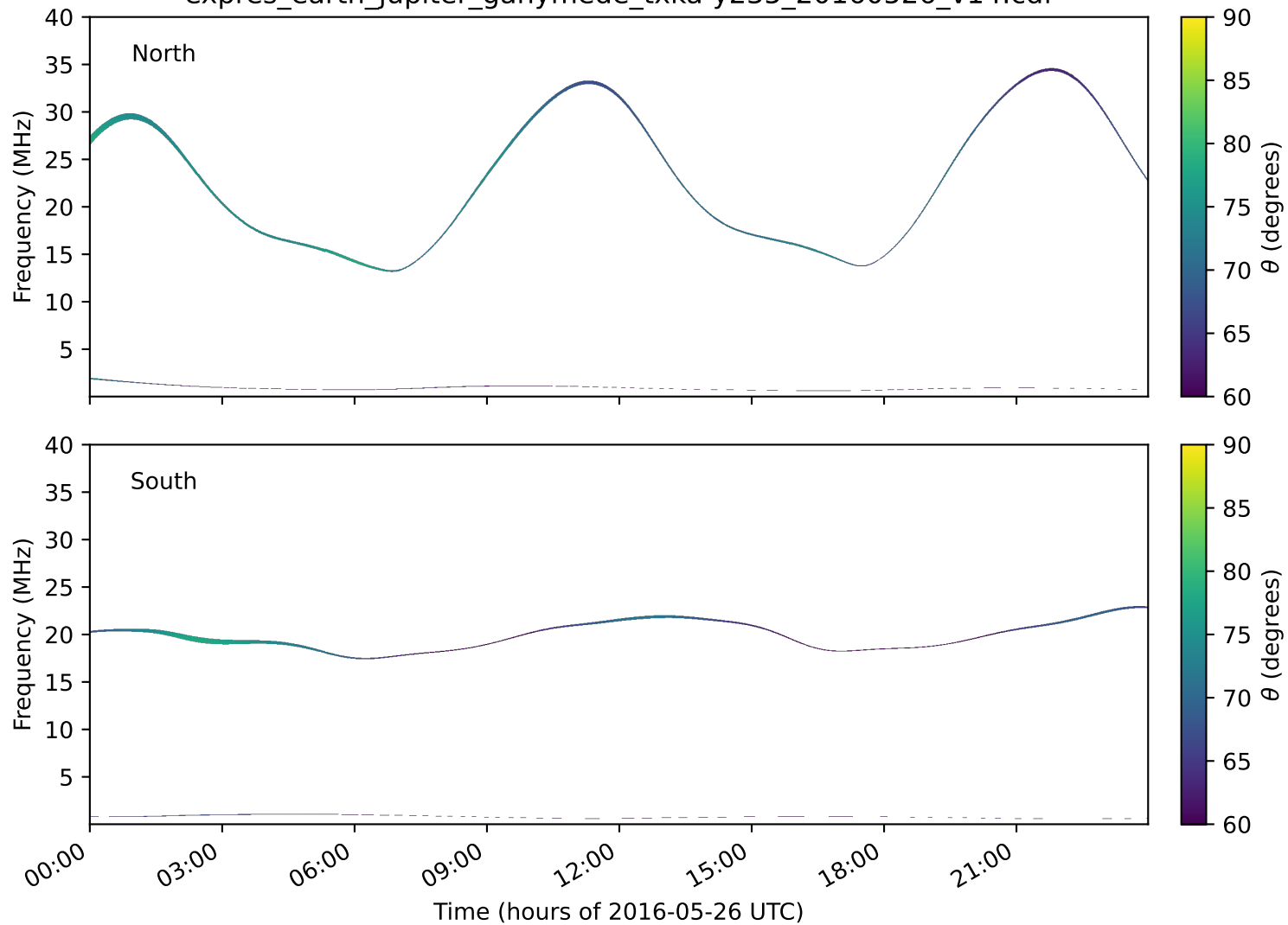
expres_earth_jupiter_ganymede_txka-y235_20160526_v14.cdf
