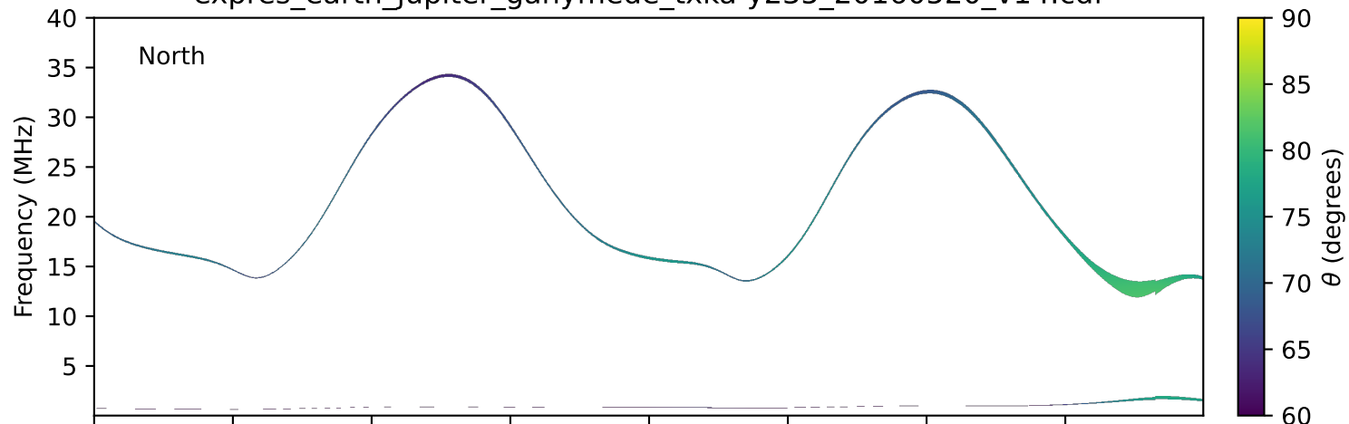
expres_earth_jupiter_ganymede_txka-y235_20160520_v14.cdf
