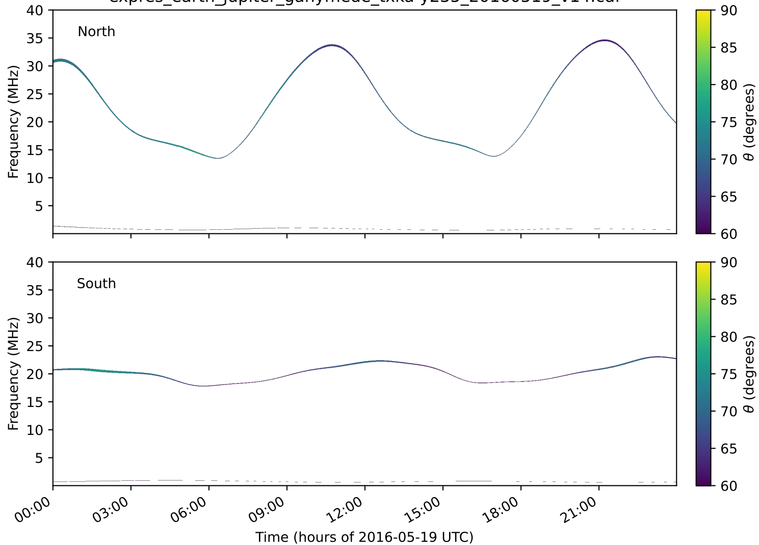
expres_earth_jupiter_ganymede_txka-y235_20160519_v14.cdf
