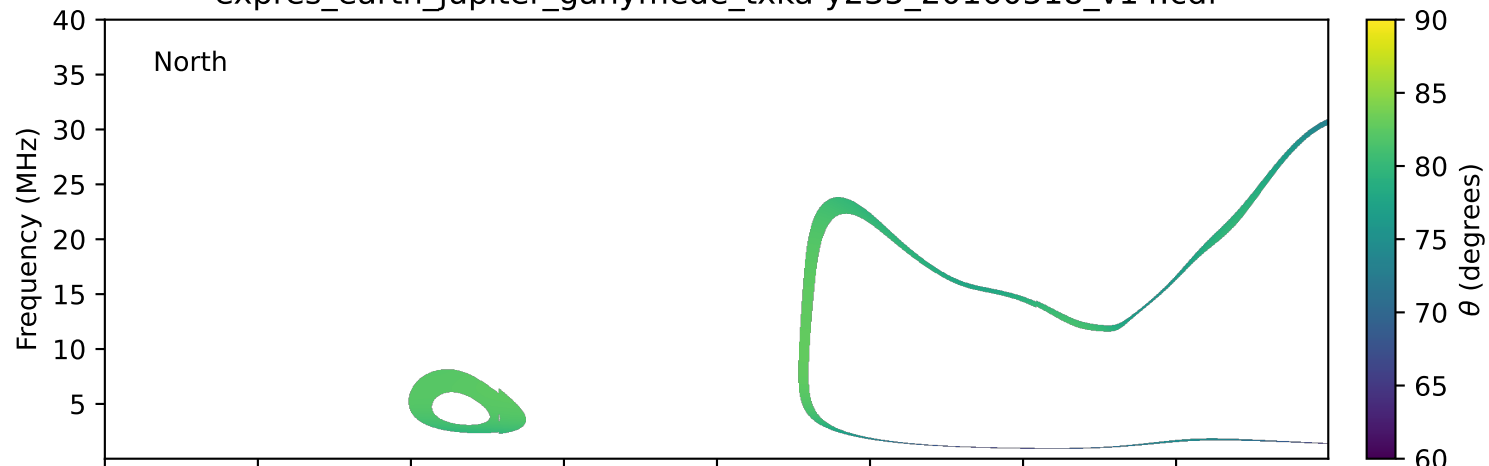
expres_earth_jupiter_ganymede_txka-y235_20160518_v14.cdf
