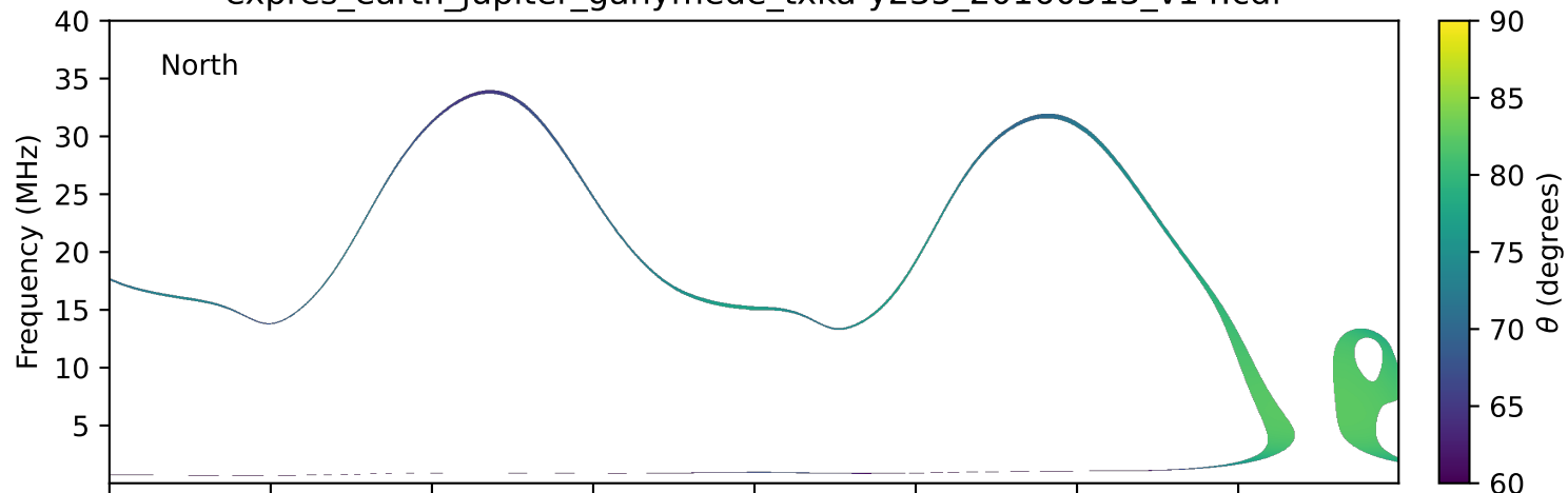
expres_earth_jupiter_ganymede_txka-y235_20160513_v14.cdf
