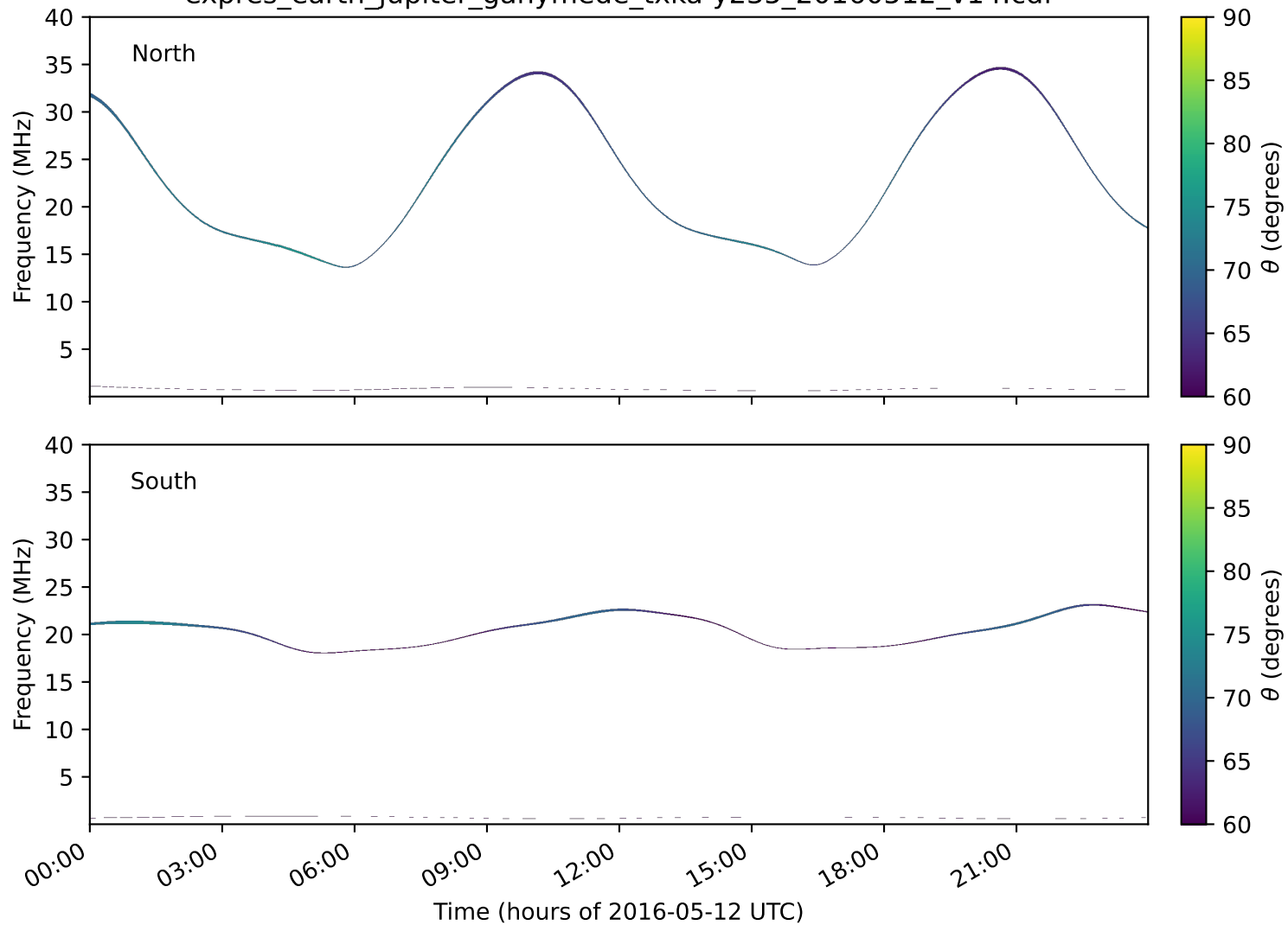
expres_earth_jupiter_ganymede_txka-y235_20160512_v14.cdf
