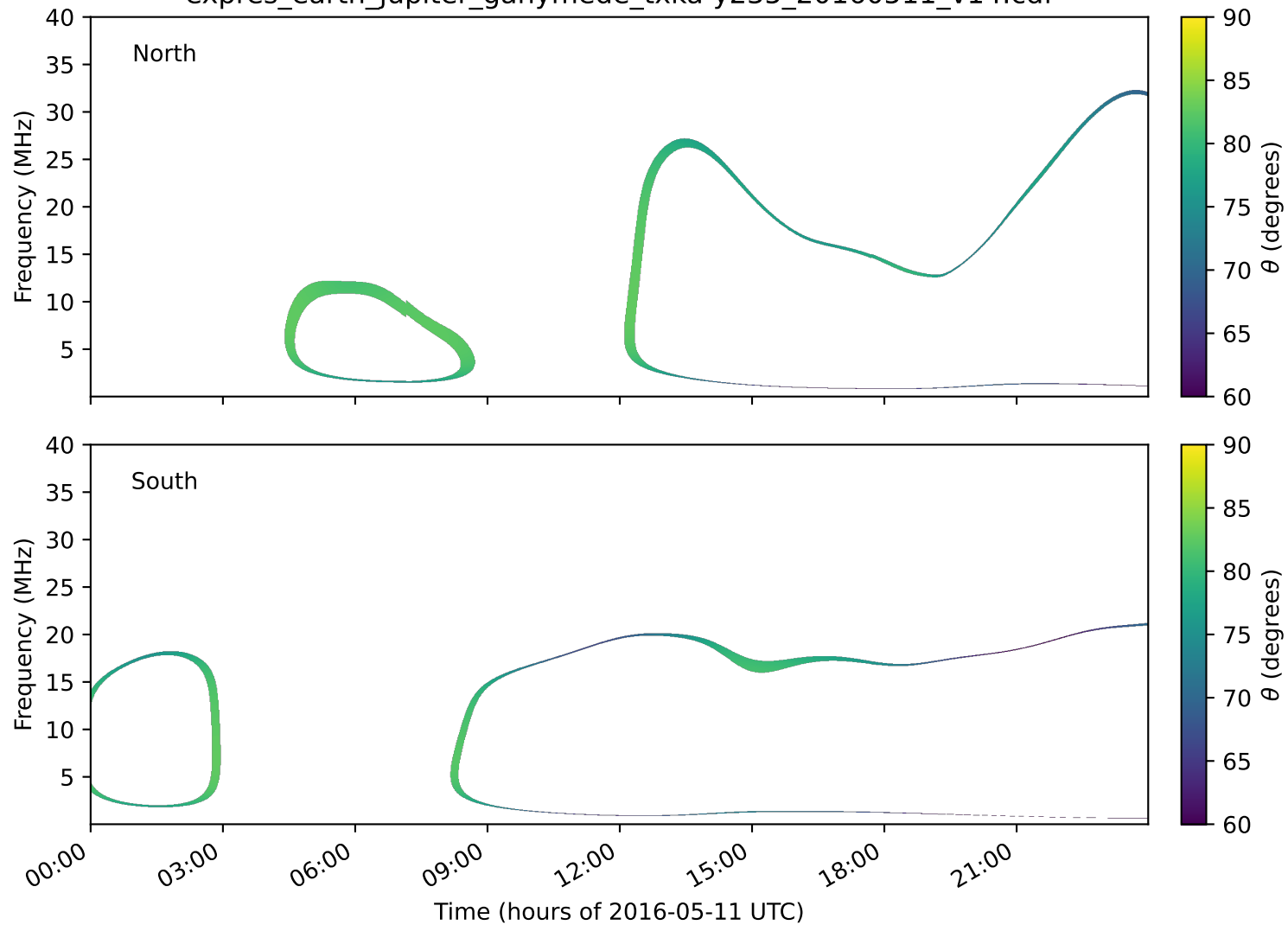
expres_earth_jupiter_ganymede_txka-y235_20160511_v14.cdf
