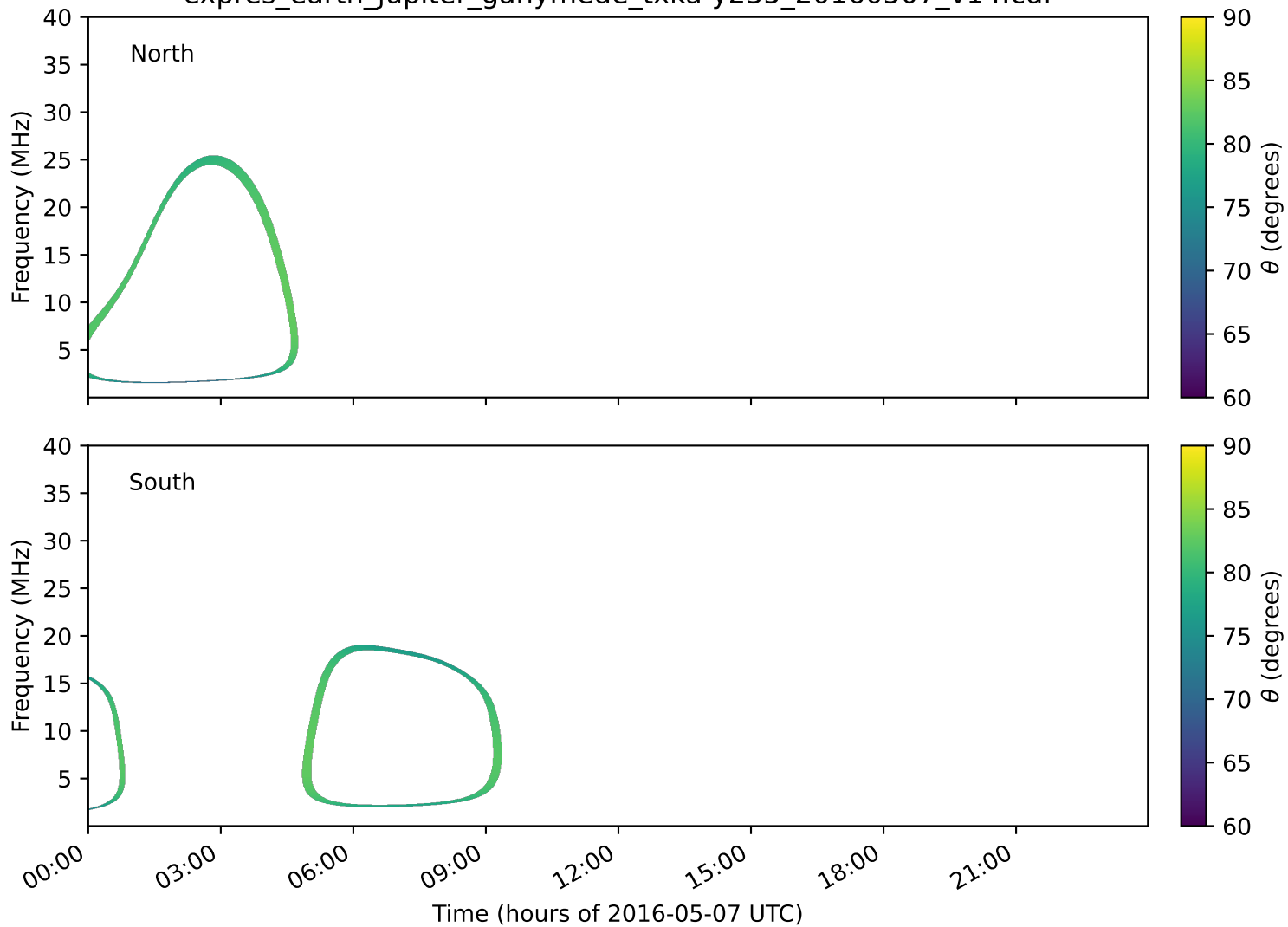
expres_earth_jupiter_ganymede_txka-y235_20160507_v14.cdf
