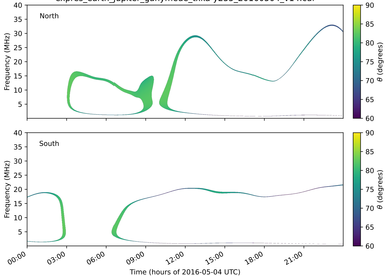
expres_earth_jupiter_ganymede_txka-y235_20160504_v14.cdf
