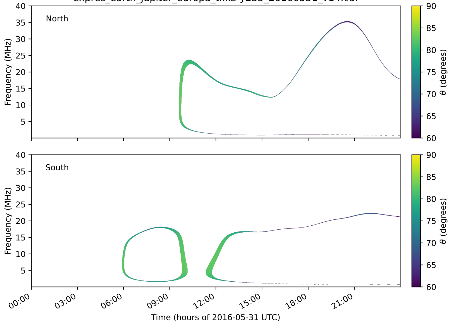
expres_earth_jupiter_europa_txka-y235_20160531_v14.cdf
