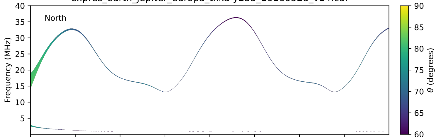
expres_earth_jupiter_europa_txka-y235_20160528_v14.cdf
