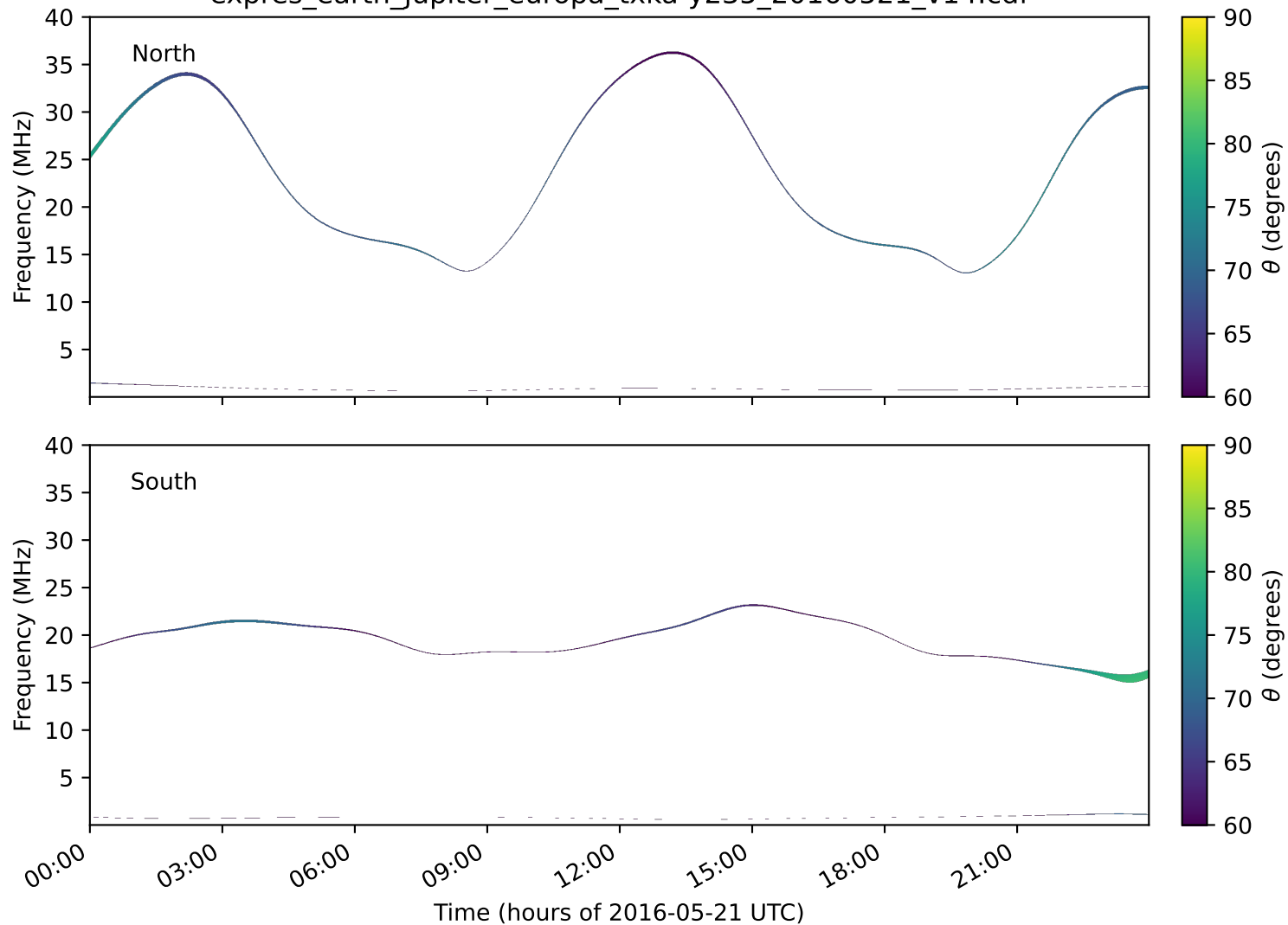
expres_earth_jupiter_europa_txka-y235_20160521_v14.cdf
