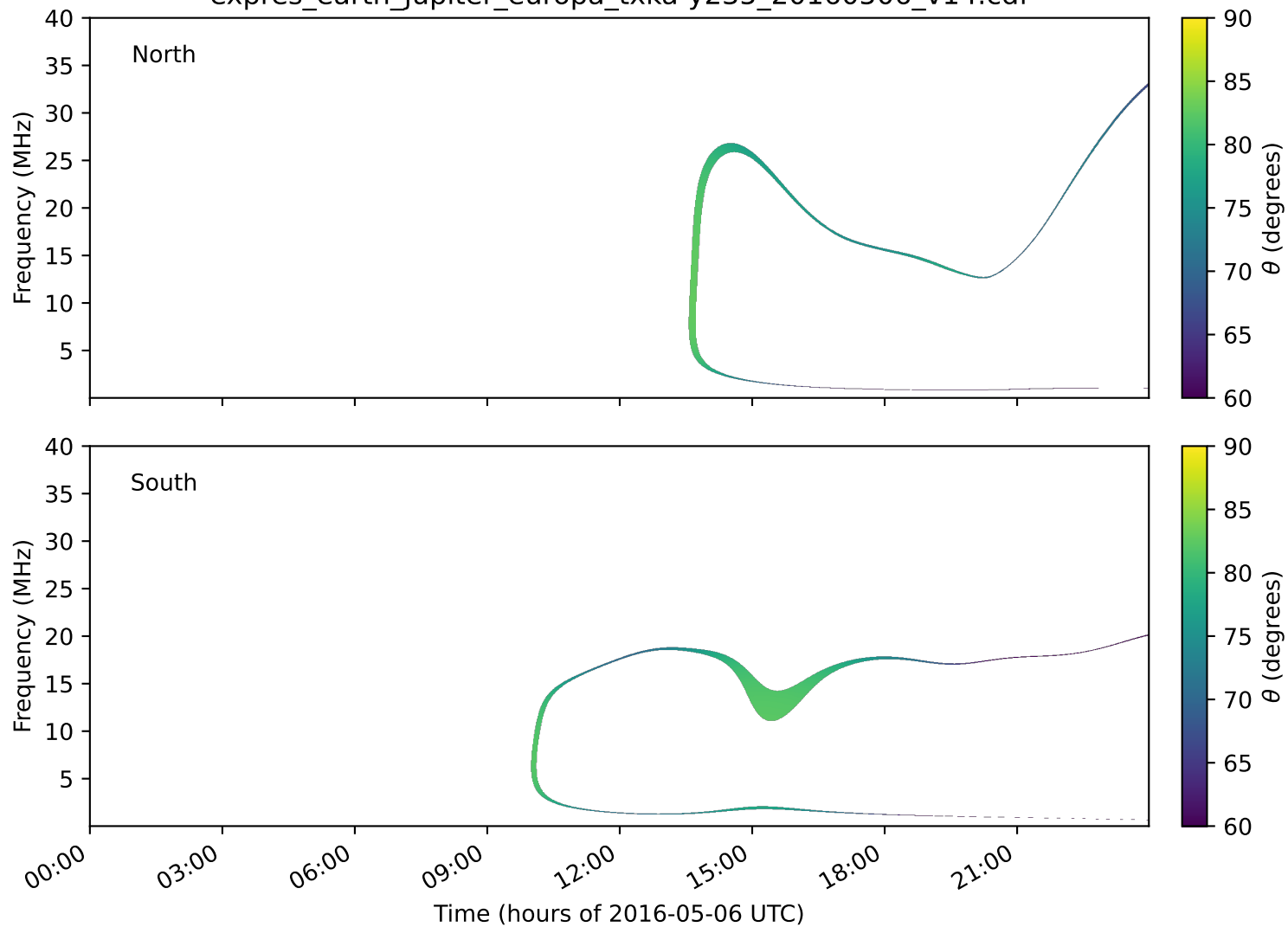
expres_earth_jupiter_europa_txka-y235_20160506_v14.cdf
