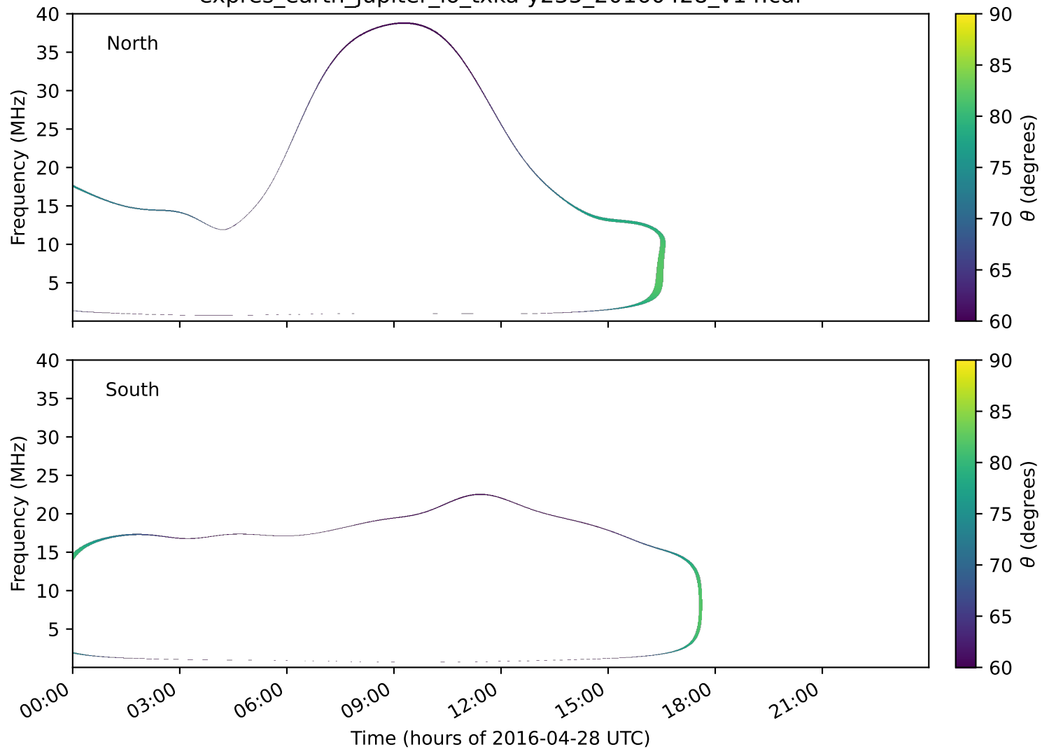
expres_earth_jupiter_io_txka-y235_20160428_v14.cdf
