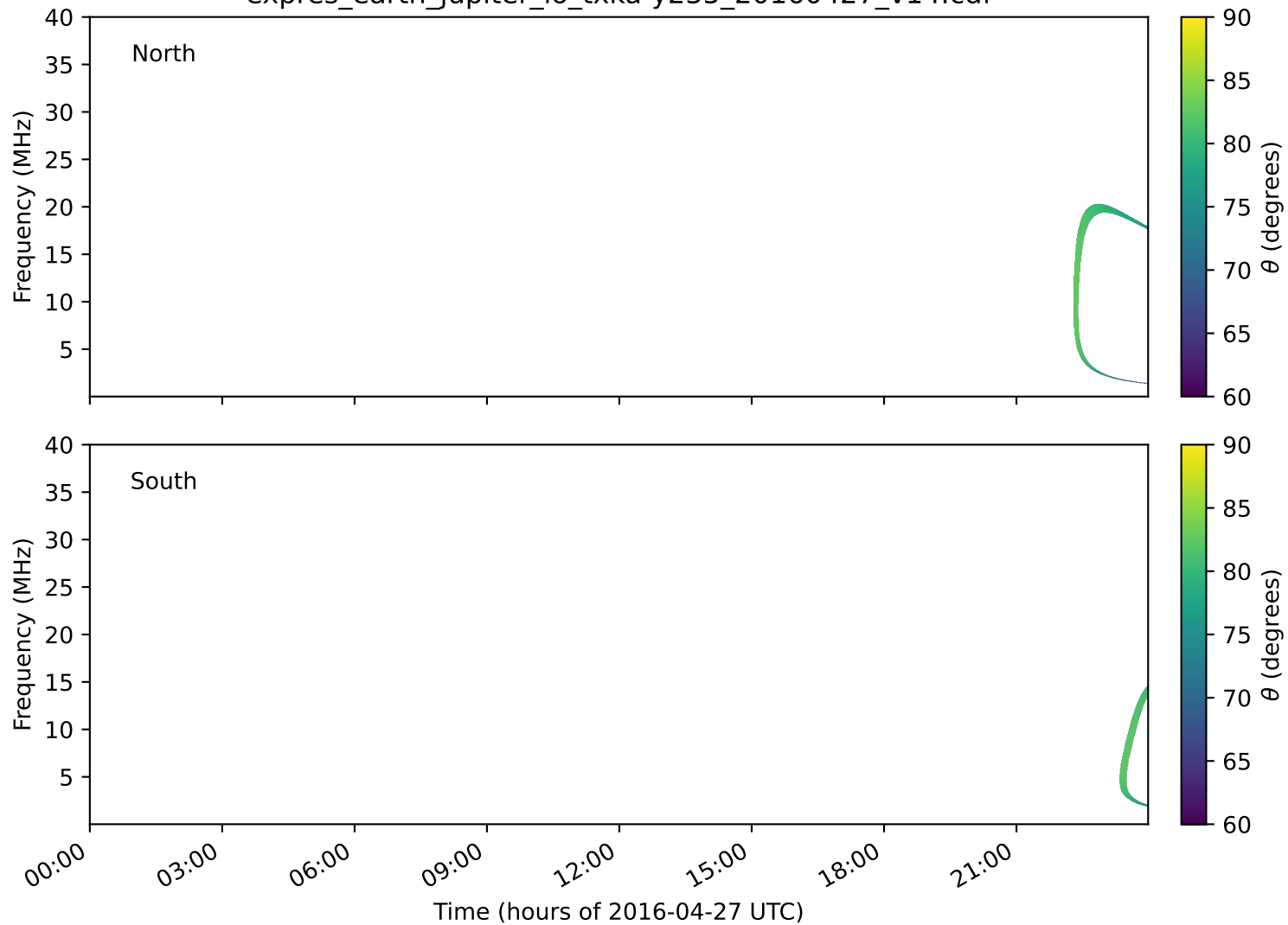
expres_earth_jupiter_io_txka-y235_20160427_v14.cdf
