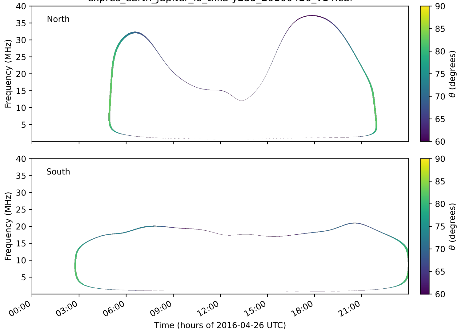
expres_earth_jupiter_io_txka-y235_20160426_v14.cdf
