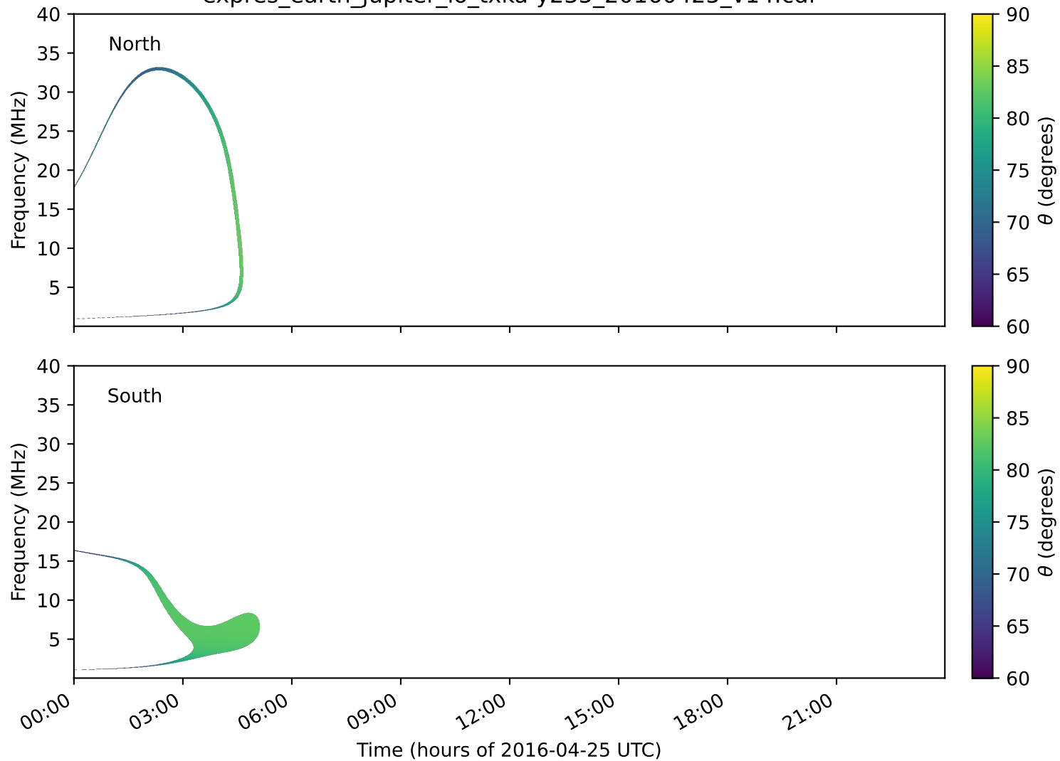
expres_earth_jupiter_io_txka-y235_20160425_v14.cdf
