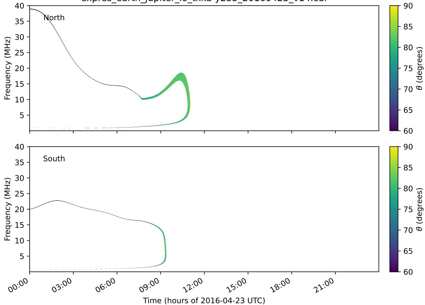
expres_earth_jupiter_io_txka-y235_20160423_v14.cdf
