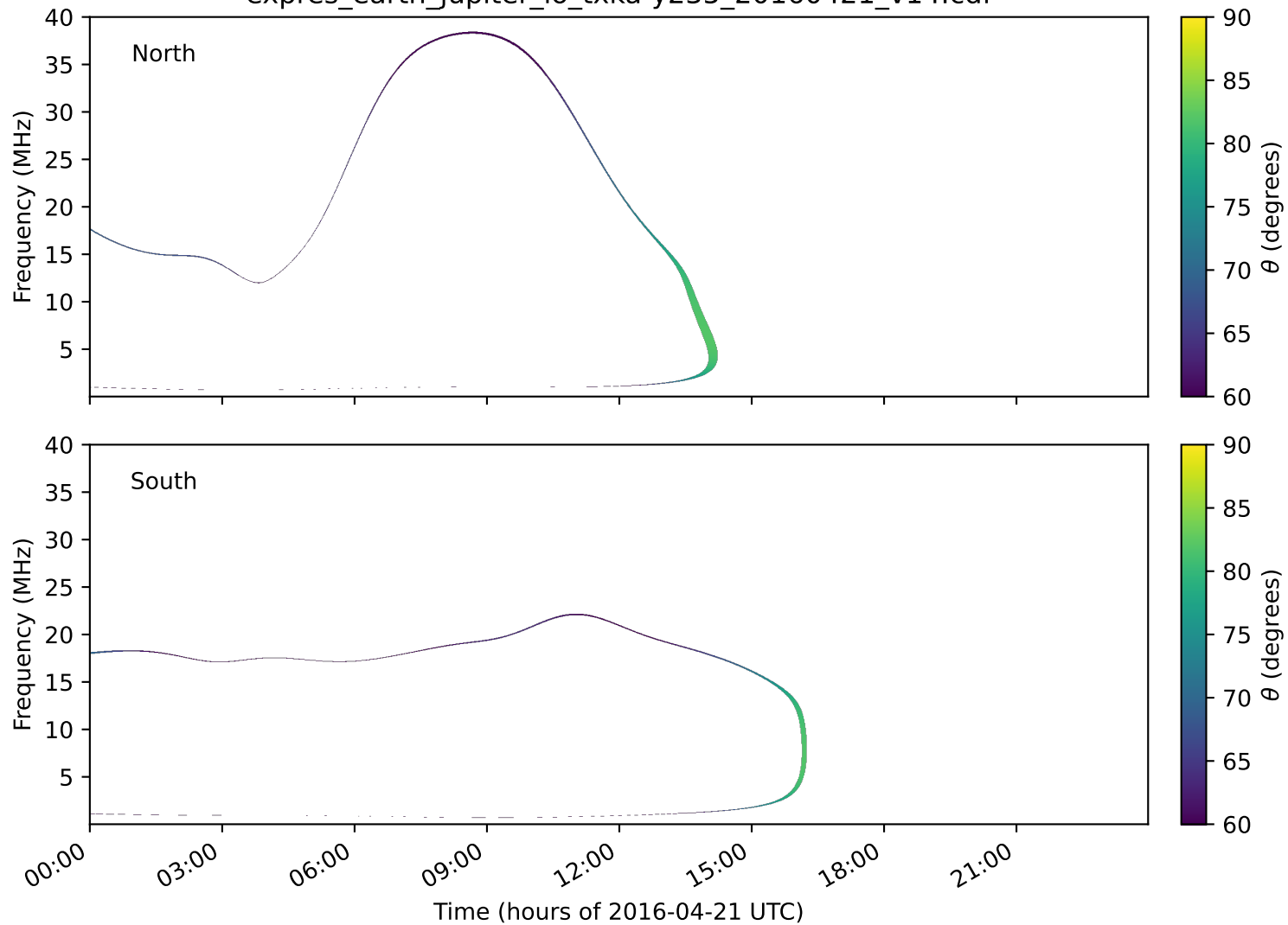
expres_earth_jupiter_io_txka-y235_20160421_v14.cdf
