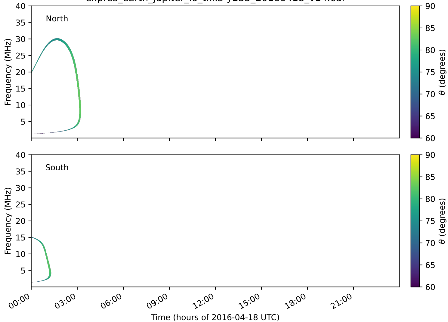
expres_earth_jupiter_io_txka-y235_20160418_v14.cdf
