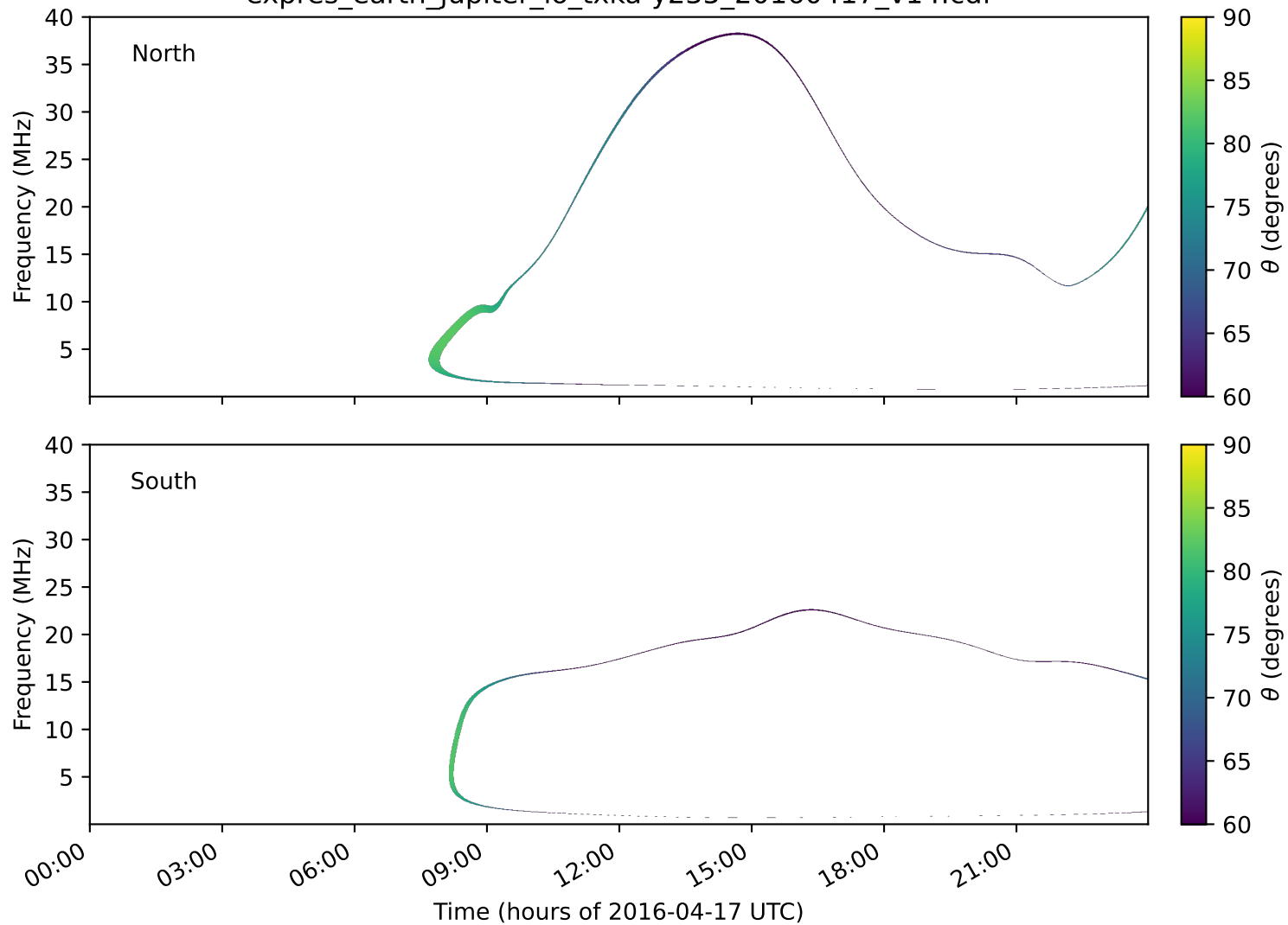
expres_earth_jupiter_io_txka-y235_20160417_v14.cdf
