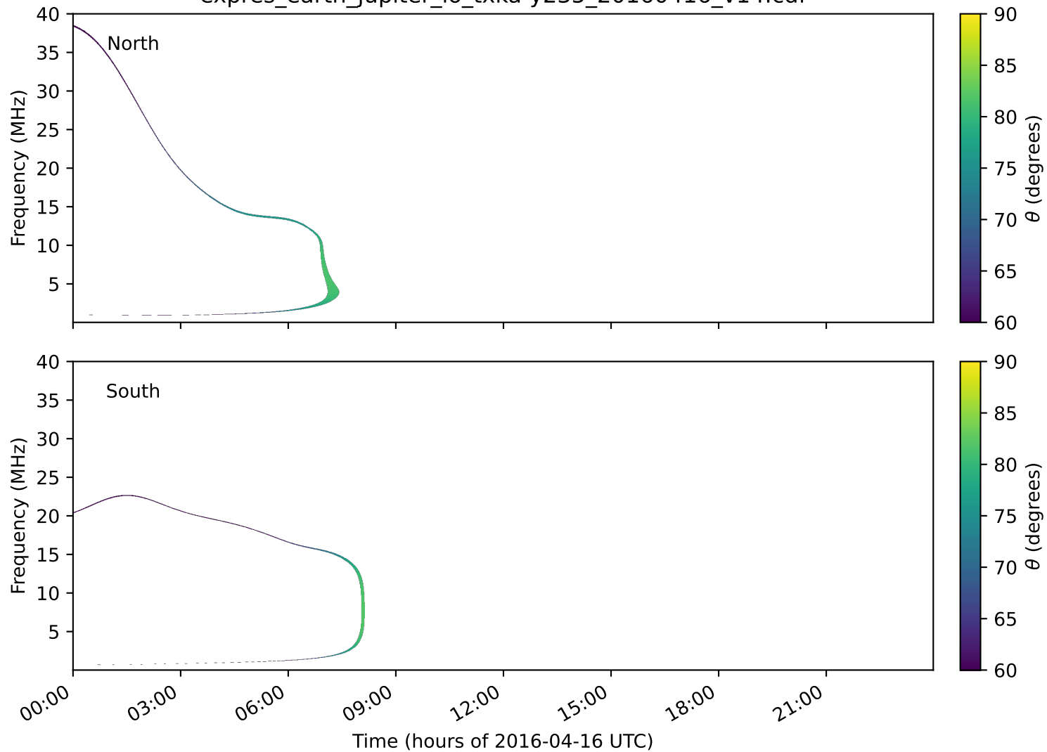
expres_earth_jupiter_io_txka-y235_20160416_v14.cdf
