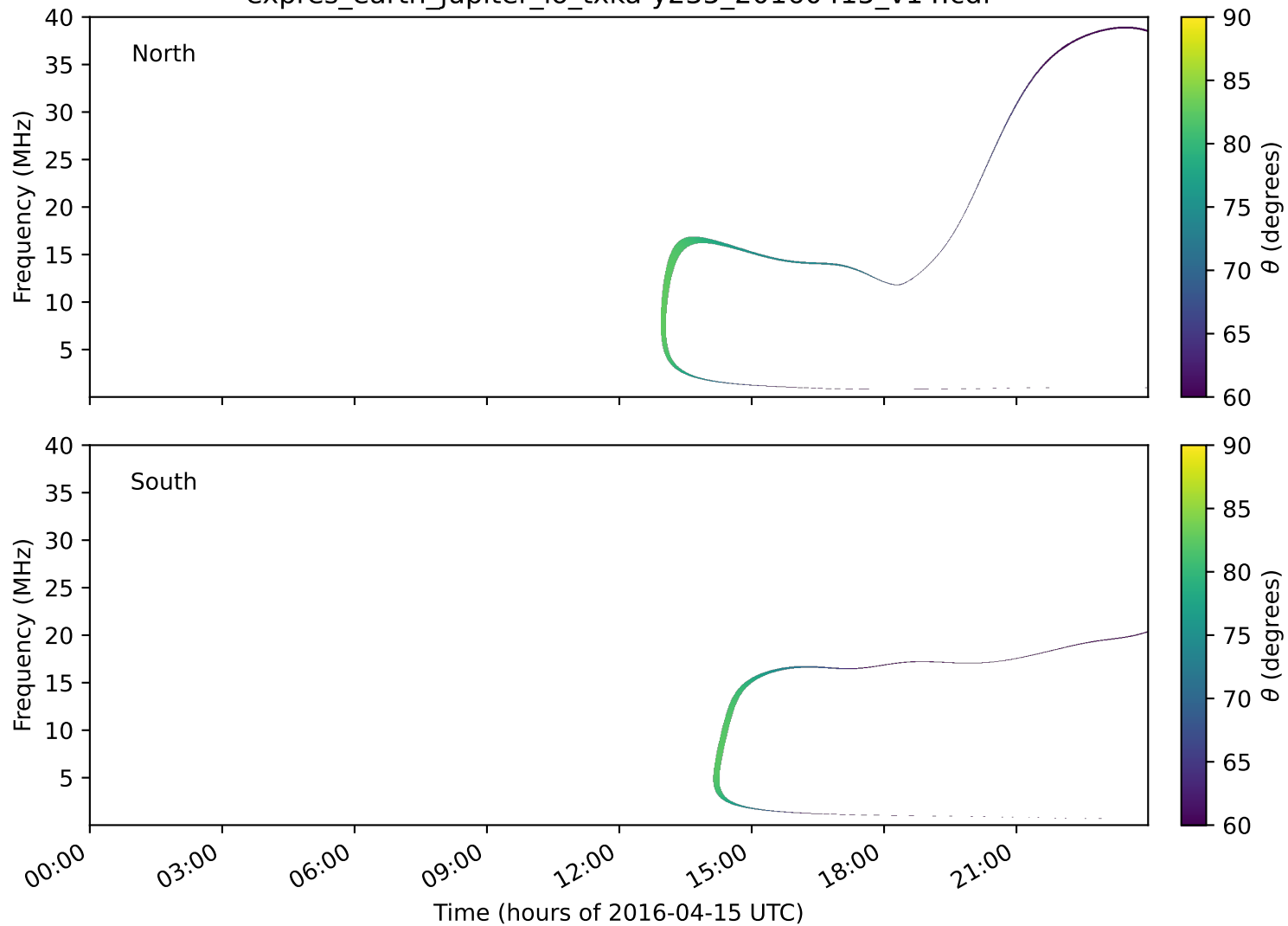
expres_earth_jupiter_io_txka-y235_20160415_v14.cdf
