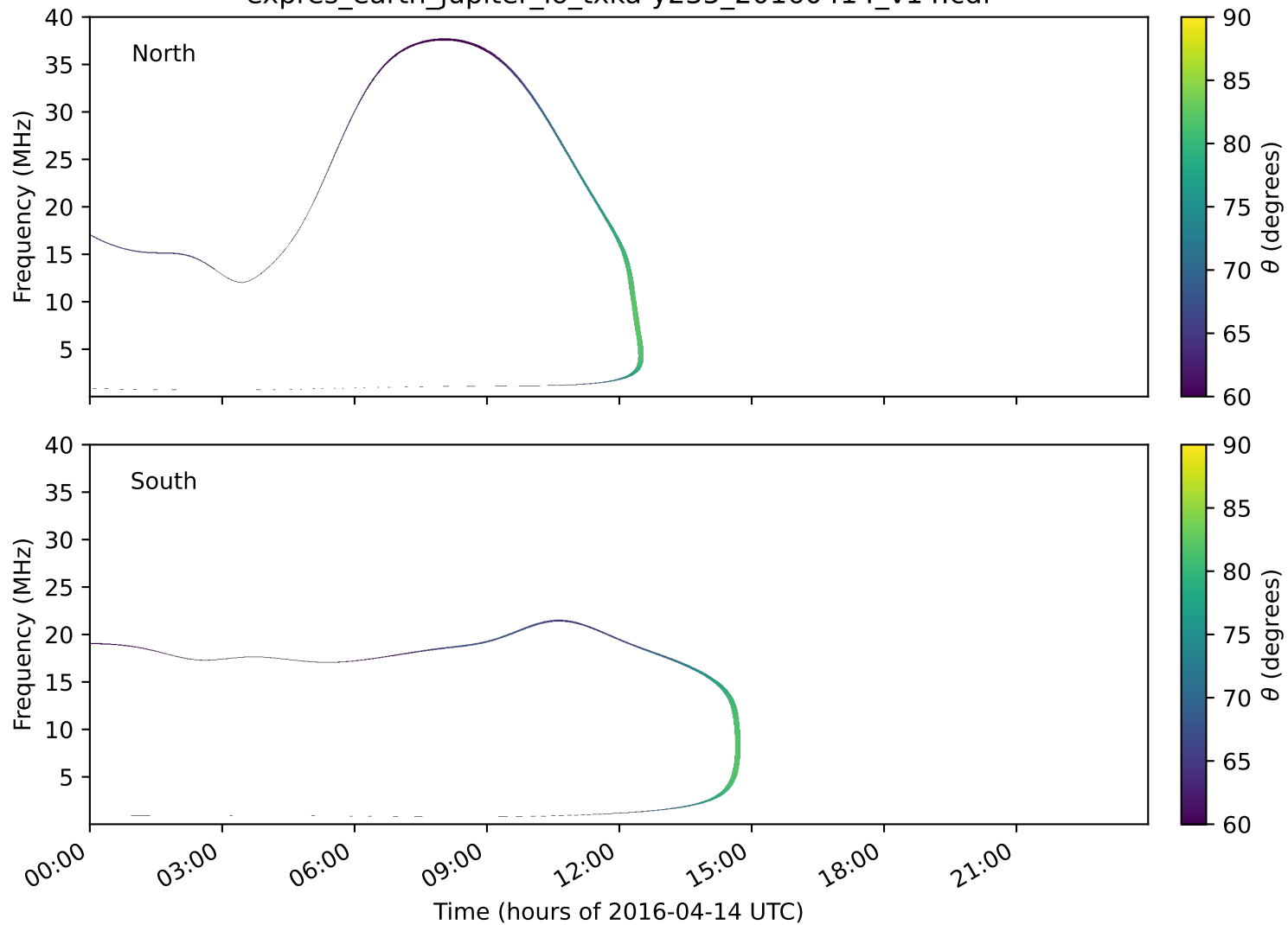
expres_earth_jupiter_io_txka-y235_20160414_v14.cdf
