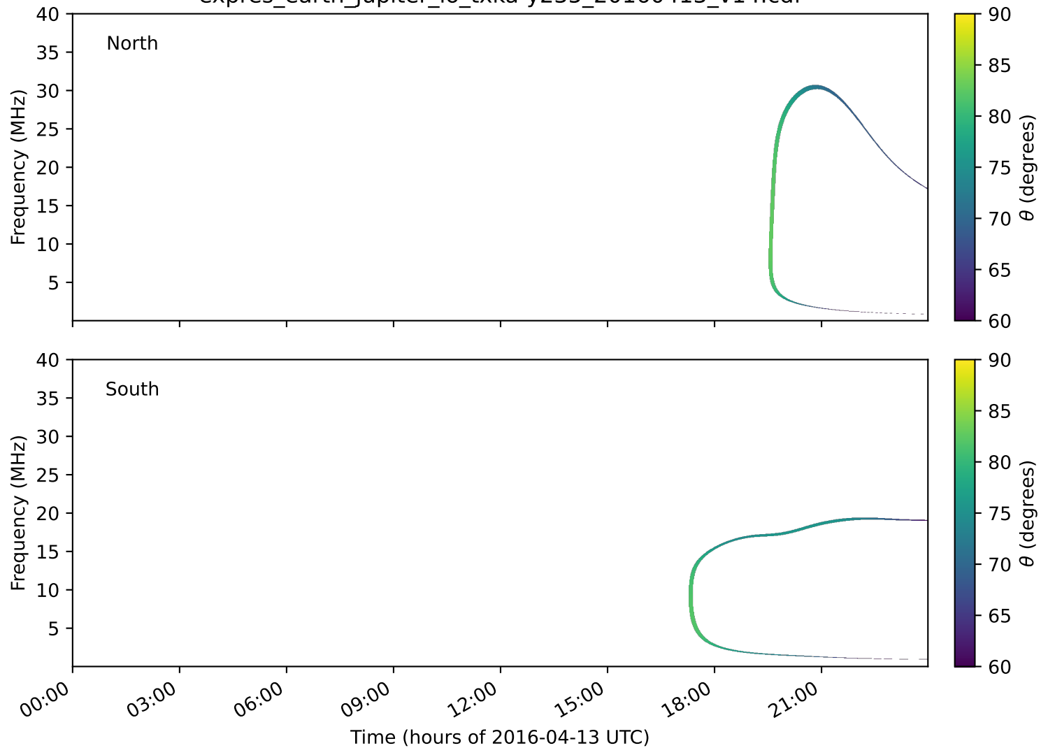
expres_earth_jupiter_io_txka-y235_20160413_v14.cdf
