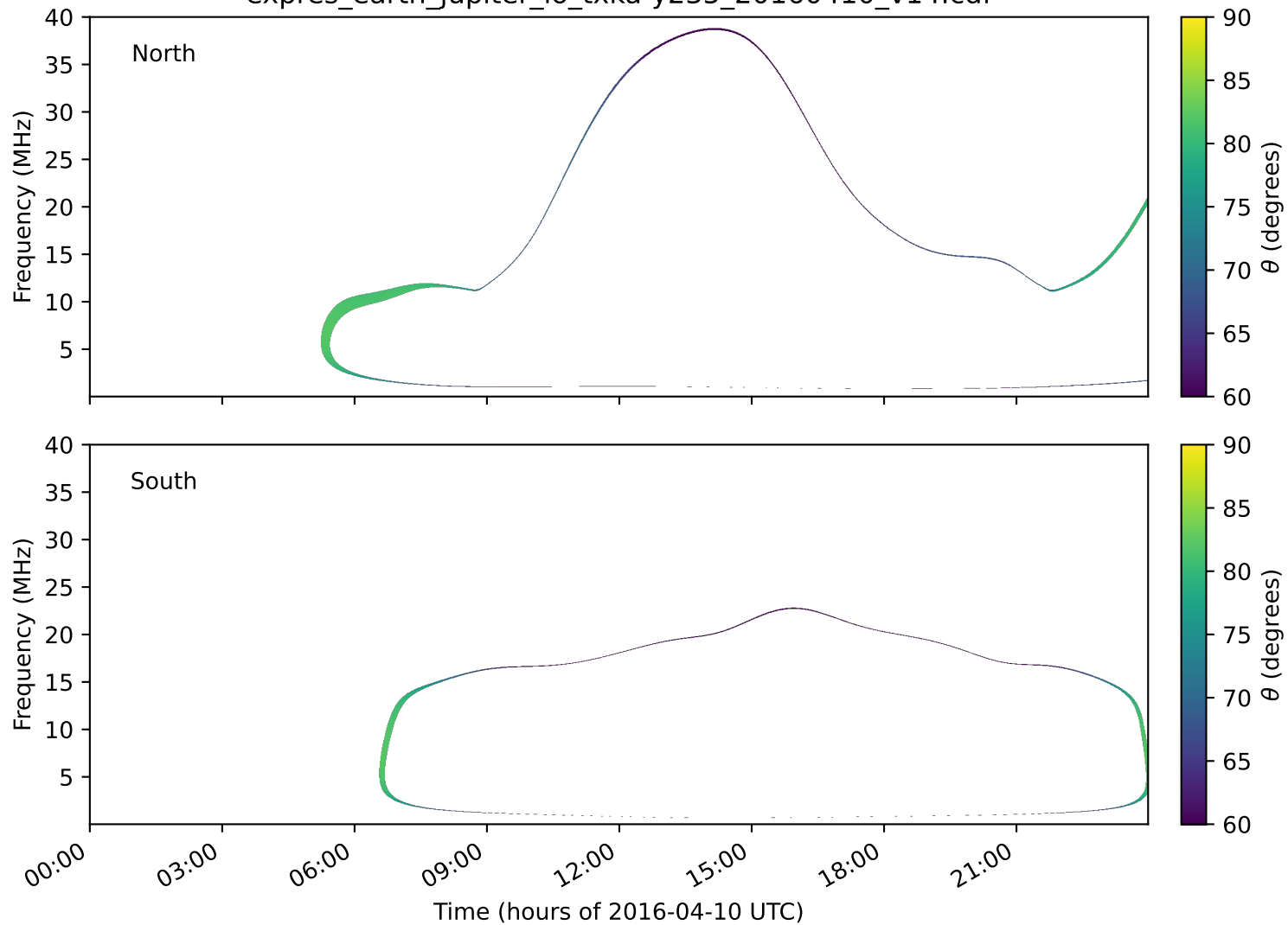
expres_earth_jupiter_io_txka-y235_20160410_v14.cdf
