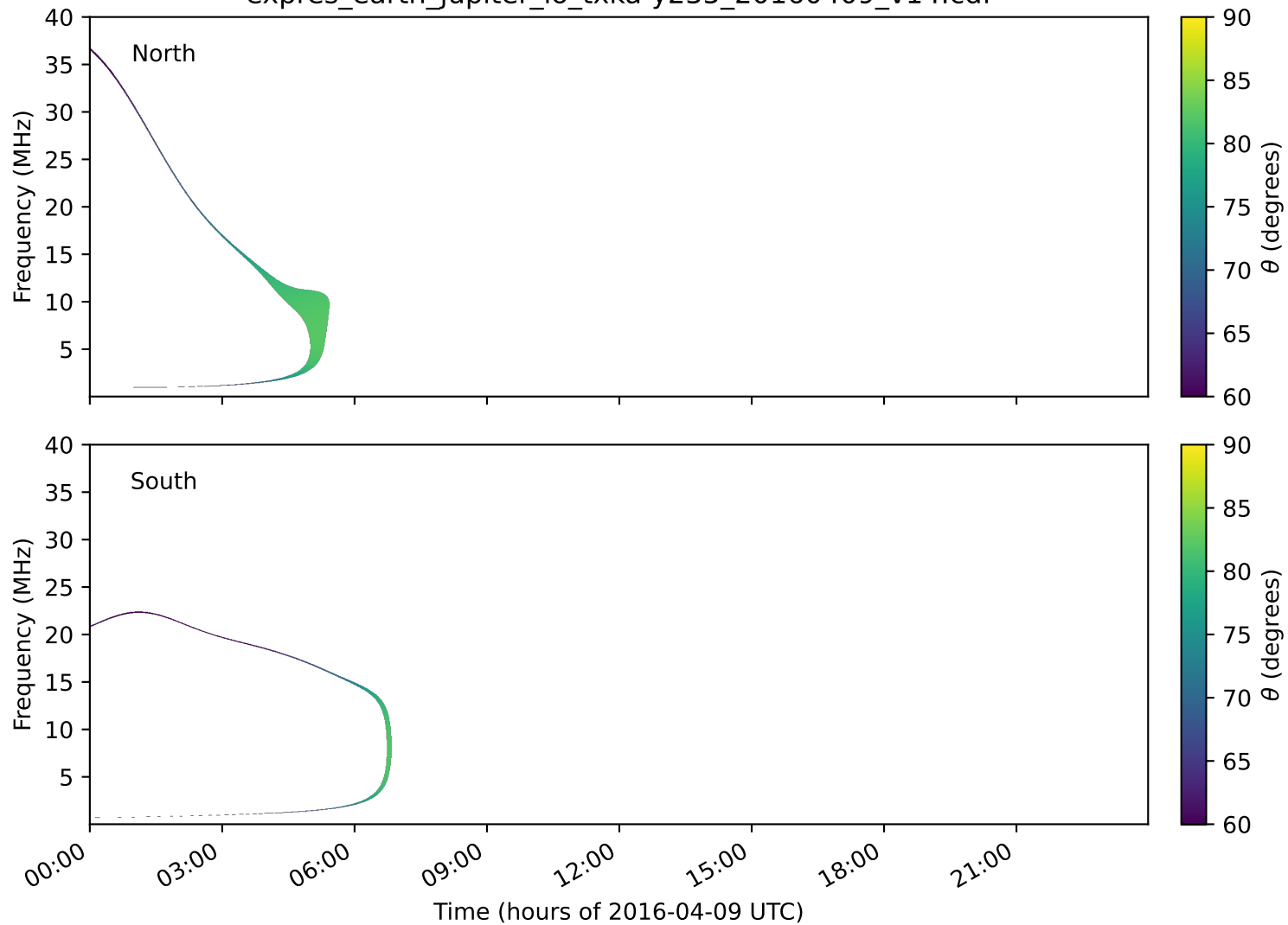
expres_earth_jupiter_io_txka-y235_20160409_v14.cdf
