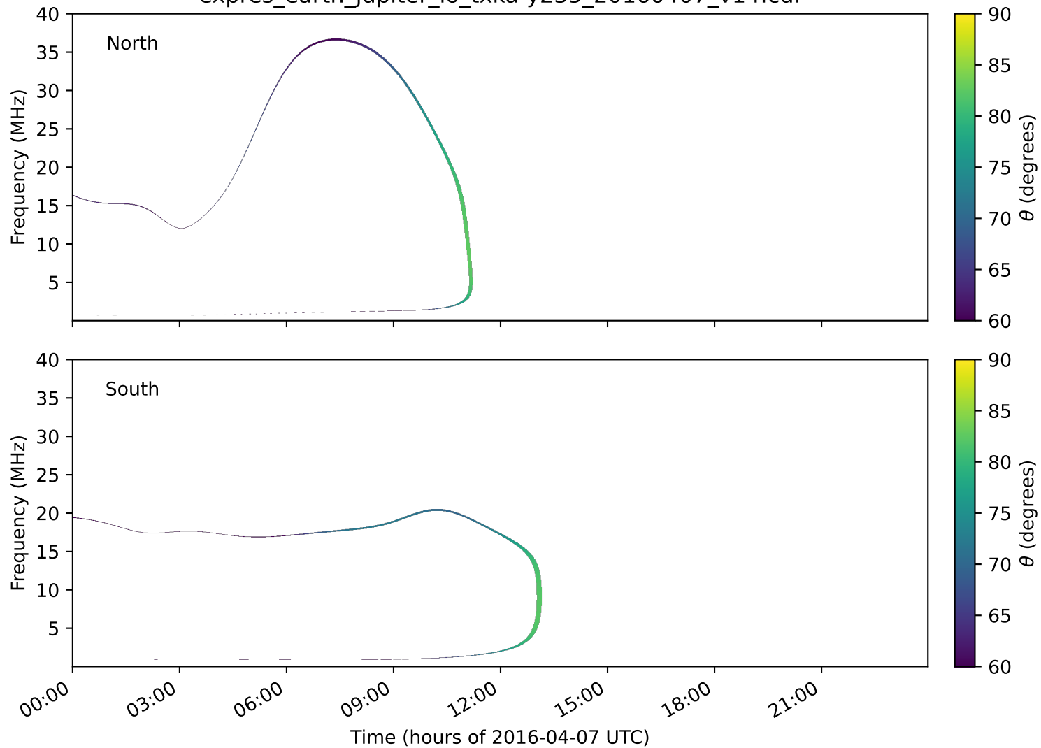
expres_earth_jupiter_io_txka-y235_20160407_v14.cdf
