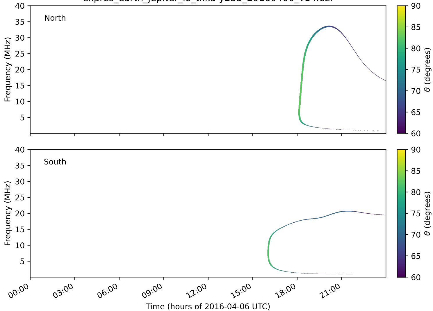
expres_earth_jupiter_io_txka-y235_20160406_v14.cdf
