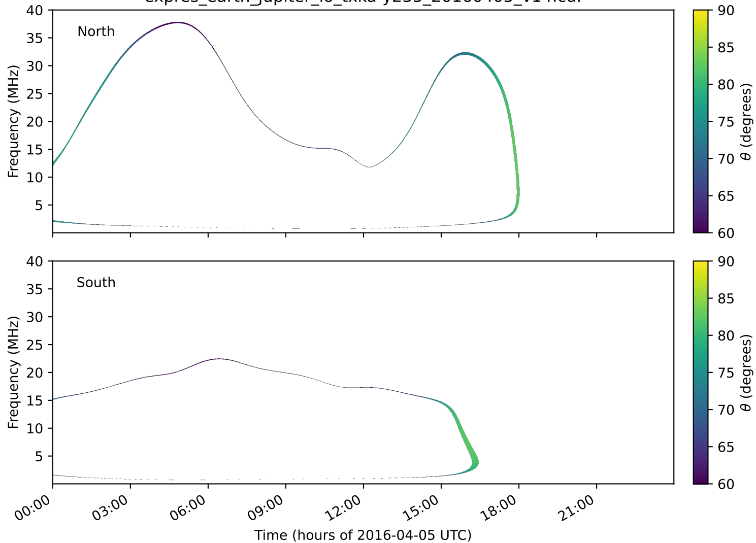
expres_earth_jupiter_io_txka-y235_20160405_v14.cdf
