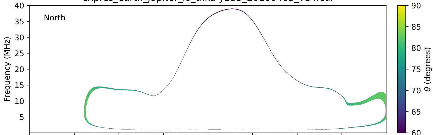
expres_earth_jupiter_io_txka-y235_20160403_v14.cdf
