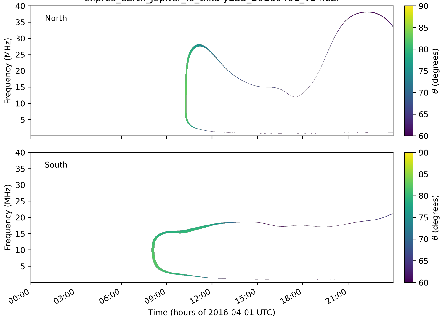
expres_earth_jupiter_io_txka-y235_20160401_v14.cdf
