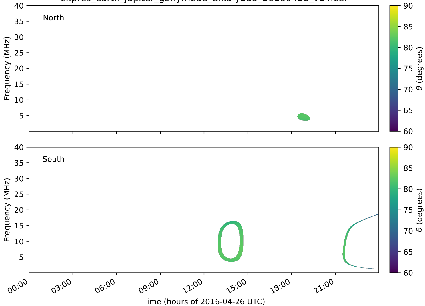
expres_earth_jupiter_ganymede_txka-y235_20160426_v14.cdf
