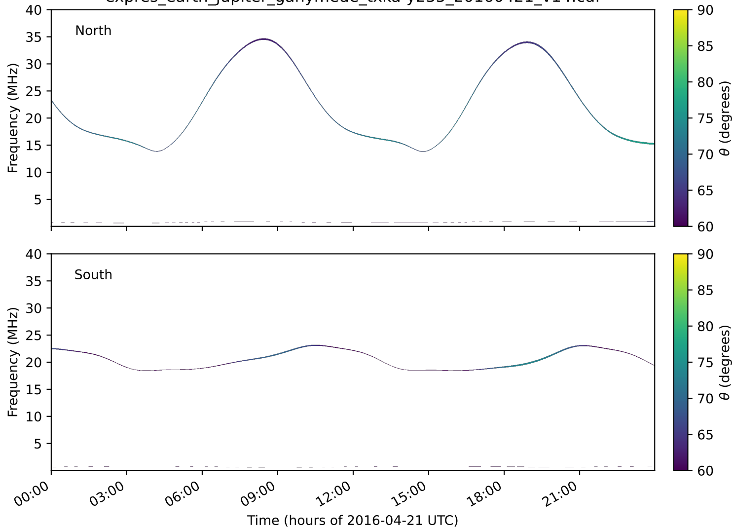
expres_earth_jupiter_ganymede_txka-y235_20160421_v14.cdf
