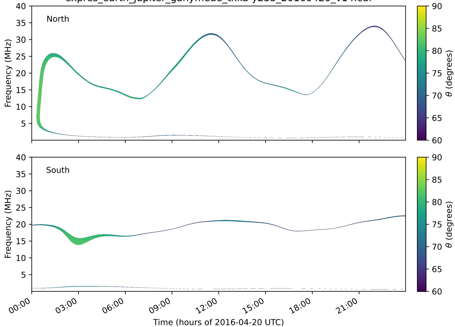
expres_earth_jupiter_ganymede_txka-y235_20160420_v14.cdf
