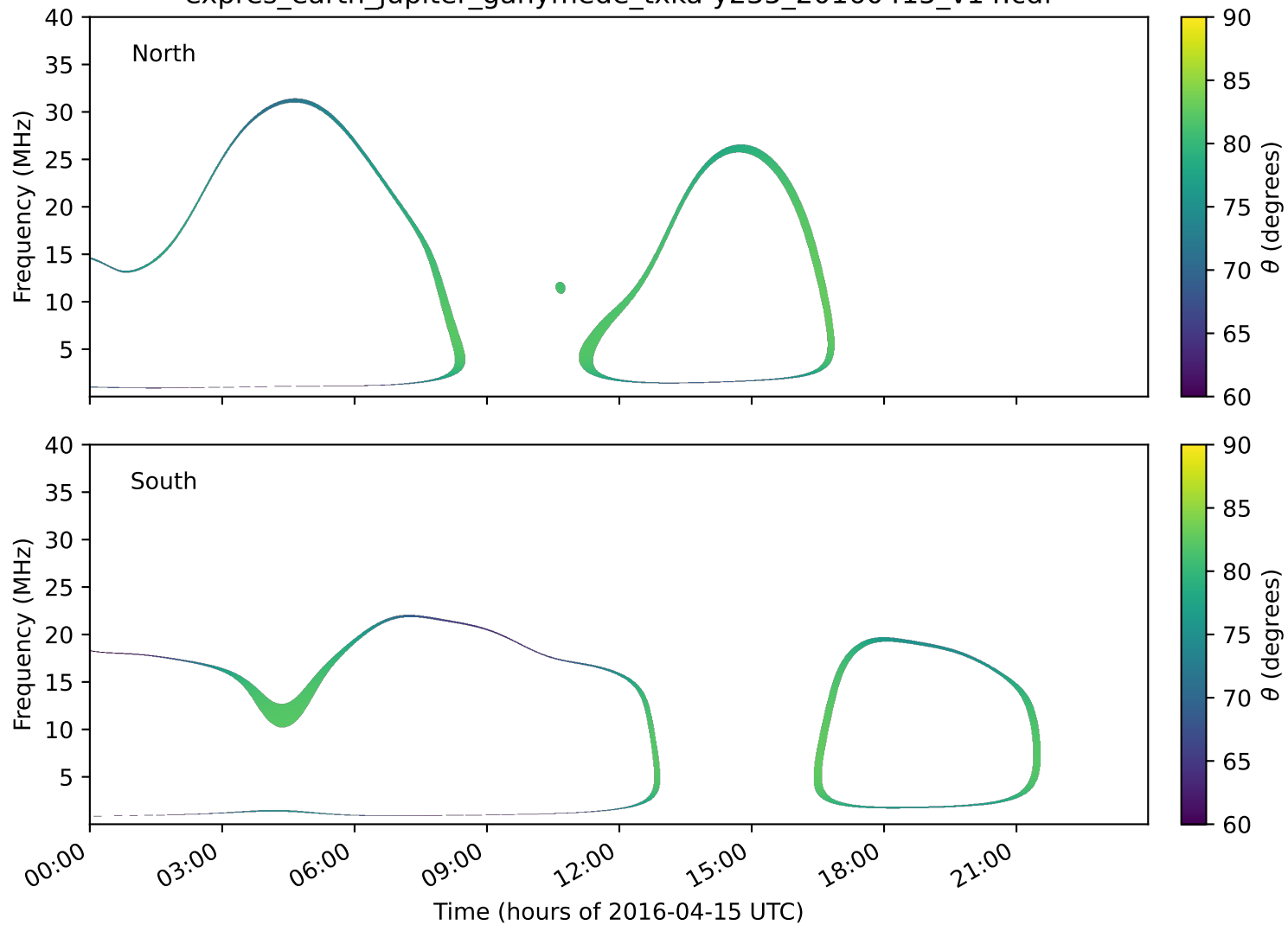
expres_earth_jupiter_ganymede_txka-y235_20160415_v14.cdf
