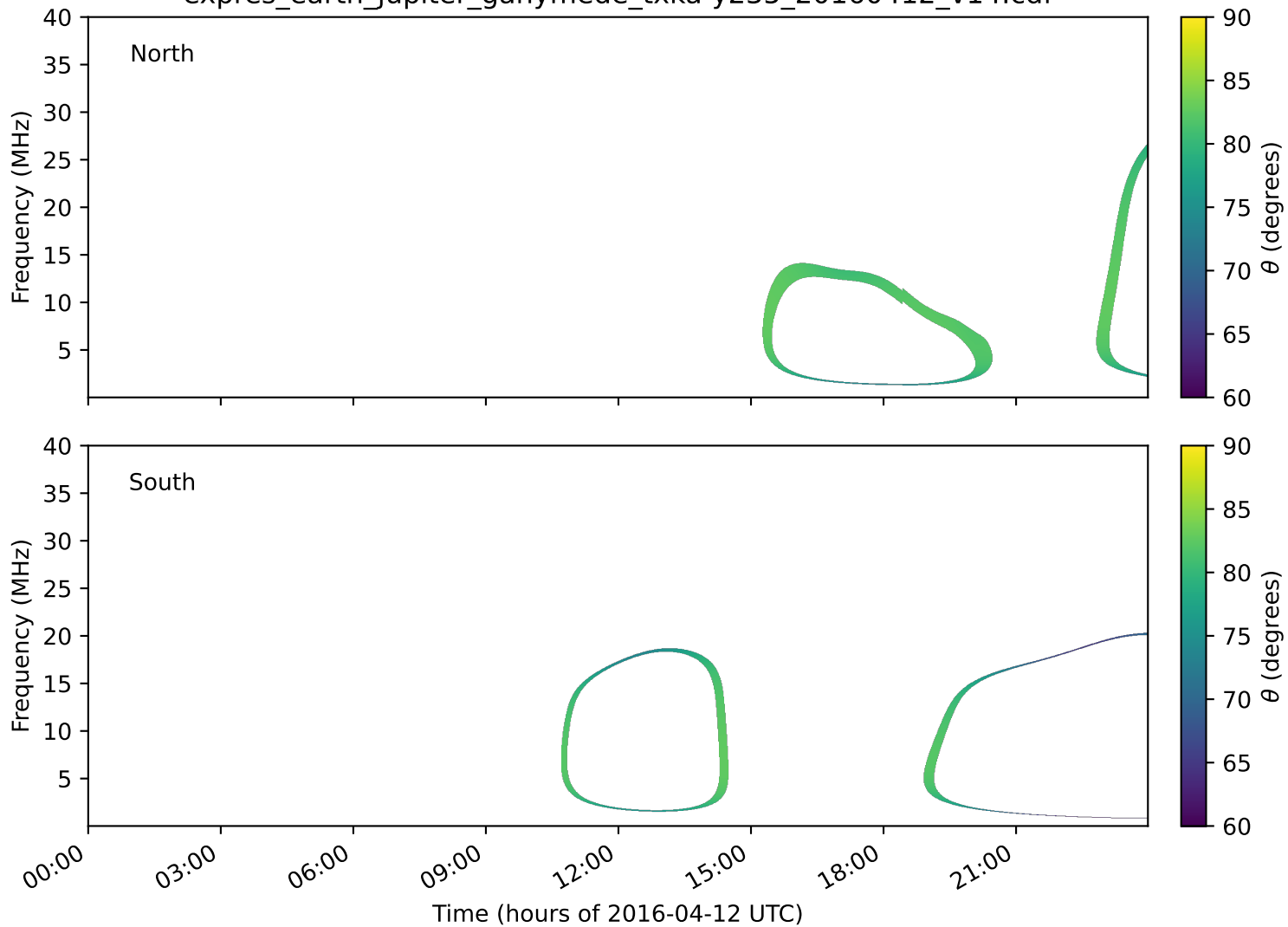
expres_earth_jupiter_ganymede_txka-y235_20160412_v14.cdf
