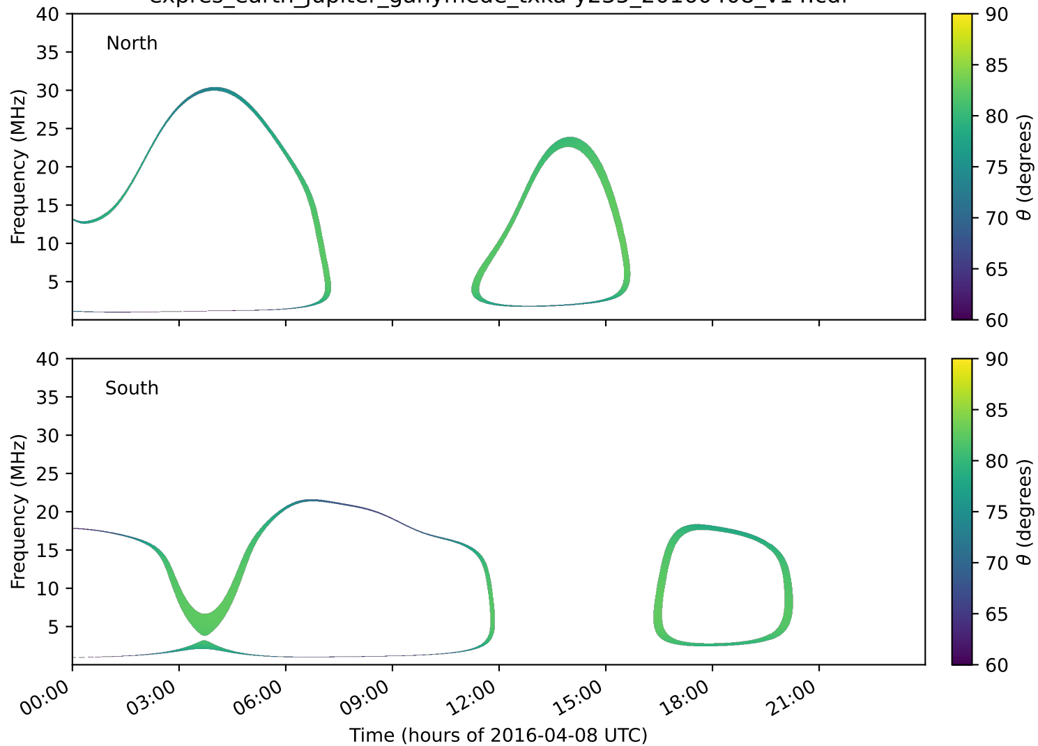
expres_earth_jupiter_ganymede_txka-y235_20160408_v14.cdf
